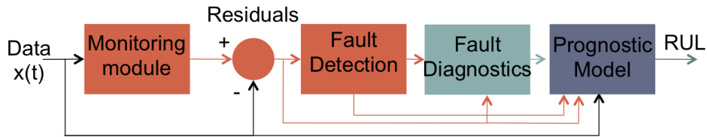
Figure 3: Combined Monitoring and Prognostic System
