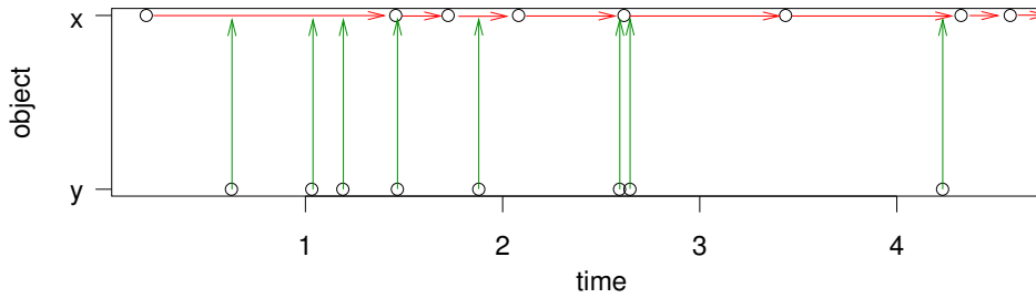
Figure 8: Matching two time sequences, assuming x reflects time intervals, and y reflects time instances. Note that the last interval extends the last time instance of x .
