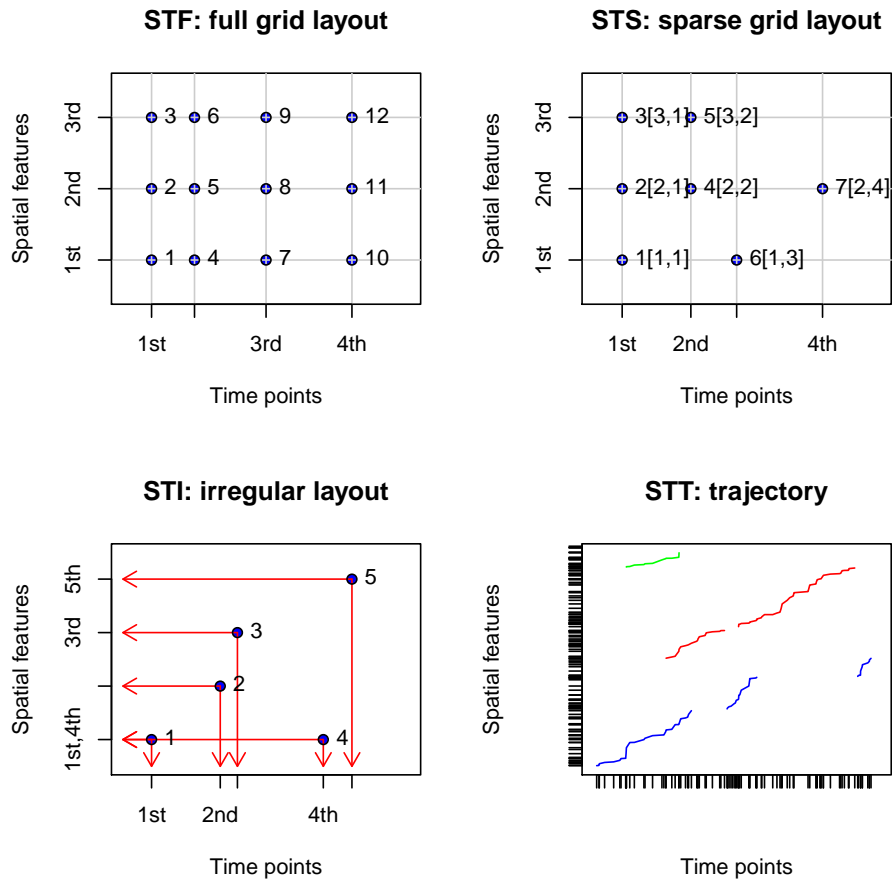
Figure 1: Four space-time layouts. Top left: Full grid (STF) layout stores all space-time combinations. Top right: The sparse grid (STS) layout stores only the non-missing space-time combinations on a lattice. Bottom left: The irregular (STI) layout: each observation has its spatial feature and time stamp stored, in this example, spatial feature 1 is stored twice – the fact that observations 1 and 4 have the same feature is not registered. Bottom right: Simple trajectories (STT), plotted against a common time axis. It should be noted that in both gridded layouts the grid is in space-time, meaning that spatial features can be gridded, but can also be any other non-gridded type (lines, points, polygons).
