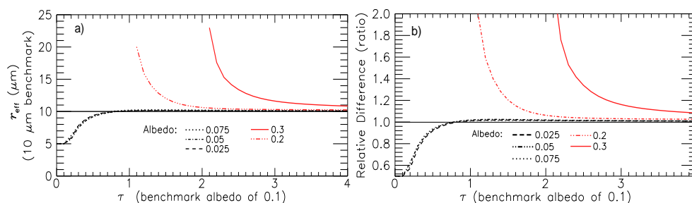
Fig. 9. (a) Absolute and (b) relative difference (ratio) between the result of a retrieval of r_{\text{eff}} and the given values and a benchmark crystal size of 10\ \mu\text{m} derived by creating a cirrus with optical thicknesses between 0 and 4, a fixed surface albedo of 0.1 and the same retrieval assuming a surface albedo of 0.025, 0.05, 0.075, 0.2 and 0.3.
