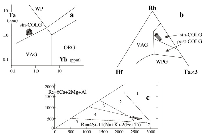
Fig. 12. Diagrams for granite geotectonic setting determination: a) Ta–Yb (Pearce et al., 1984.), b) Rb–Hf–Tax3 (Harris et al., 1986), c) R_1 – R_2 (Batchelor & Bowden, 1985) with marked positions of the Polumir granites. Explanation: a–b) granites; WPG–Within Plates, ORG– Ocean Ridges, VAG– Volcanic arc, Sin–COLG– Sin–Collision, Post–COLG– Post–Collision; c) 1– Mantle–Fractionates, 2– Pre–Plate Collision, 3– Post–Collision Uplif, 4– Late–Orogenic, 5– Anorogenic, 6– Sin–Collision, 7– Post–Orogenic.
