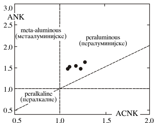
Fig. 2. The ACNK-ANK diagram (Maniar & Piccoli, 1989) for the Polumir granites.
