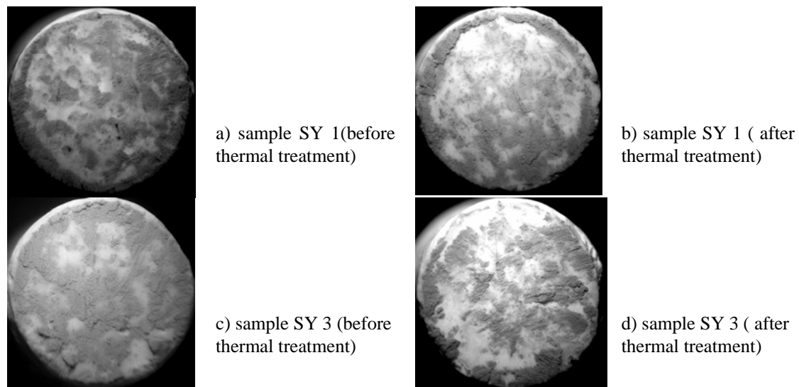
Fig. 1 Photographs of samples under thermal shock experiment, white area is non damaged surface, dark area is damaged surface
