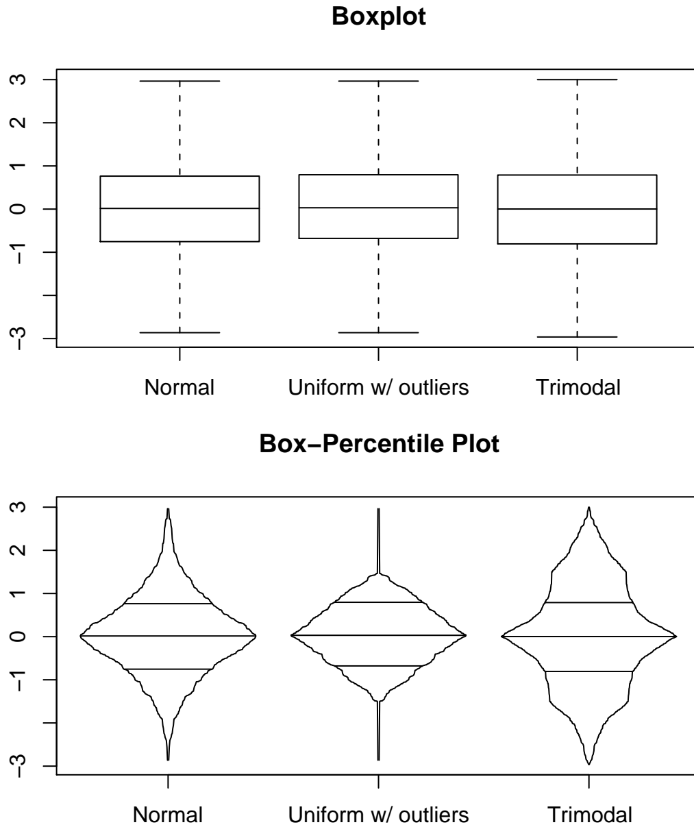
Figure 3: Boxplots and box-percentile plots for the data sets shown in Figure 2. Although all three boxplots are essentially identical, the box-percentile plots show the three data sets are very different.
