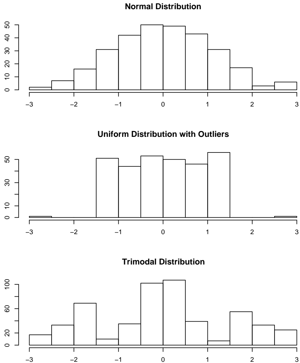
Figure 2: Histograms of three simulated data sets. Figure 3 uses these data sets to compare the effectiveness of boxplots and box-percentile plots in distinguishing between these three distinctly different distributions.
