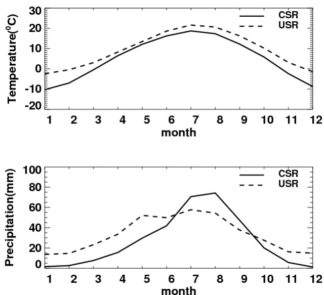
Fig. 2. Comparison of annual temperature (°C) and precipitation (mm) cycles over the CSR and USR.
