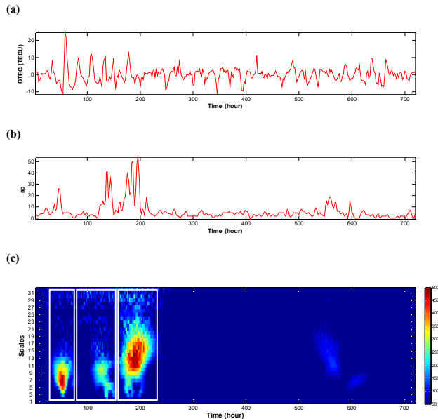
Fig. 7. (a) The DTEC time series right over the epicenter ( 30.3^{\circ} N, 103.0^{\circ} E) of the Ya'an earthquake from 22 March 2013 to 20 April 2013. (b) The variations of the ap geomagnetic index from 22 March 2013 to 20 April 2013. (c) The cross-wavelet spectrum for DTEC and ap using fbsp2-1-0.5 wavelet.
