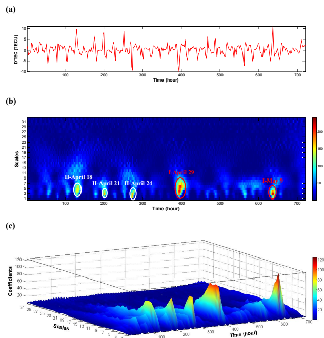
Fig. 1. (a) The DTEC time series right over the epicenter ( 31.0^{\circ} N, 103.4^{\circ} E) of the Wenchuan earthquake from 13 April to 12 May, 2008. (b) The analytic wavelet energy density spectrum of DTEC using fbsp2-1-0.5 wavelet. The thick red ellipse designates the “I” style significant enhancement. The thick white ellipse designates the “II” style significant enhancement. (c) The 3-D coefficient plots of the analytic wavelet energy density spectrum.
