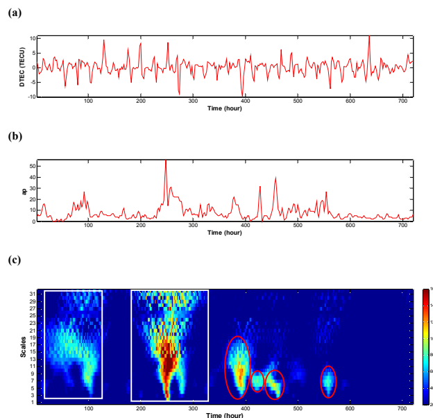
Fig. 2. (a) The DTEC time series right over the epicenter ( 31.0^{\circ} N, 103.4^{\circ} E) of the Wenchuan earthquake from 13 April to 12 May, 2008. (b) The variations of the a_p geomagnetic index from 13 April to 12 May, 2008. (c) The cross-wavelet spectrum for DTEC and a_p using fbsp2-1-0.5 wavelet.
