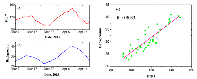
Fig. 5. (a) Solar activity index F10.7 time series. (b) Decomposed TEC background time series. (c) The Pearson correlation between the background and F10.7.
