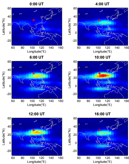
Fig. 4. Two-dimensional maps for small scales of analytic wavelet energy density spectrum on 9 May 2008 from 00:00 to 16:00 UT. The red star represents the epicenter.
