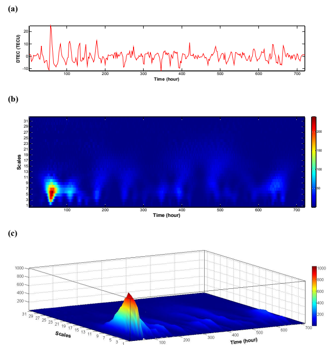
Fig. 6. (a) The DTEC time series right over the epicenter (30.3° N, 103.0° E) of the Ya’an earthquake from 22 March 2013 to 20 April 2013. (b) The analytic wavelet energy density spectrum of DTEC using fbsp2-1-0.5 wavelet. (c) The 3-D coefficient plots of the analytic wavelet energy density spectrum.
