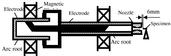
Figure (1) : Sketch of the arc heater
