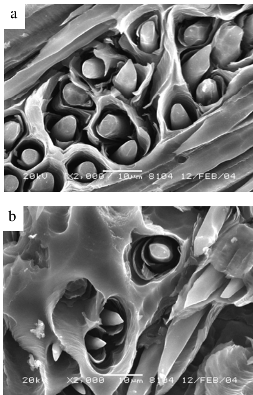
Figure (5) : Ablation morphologies of sample C.
