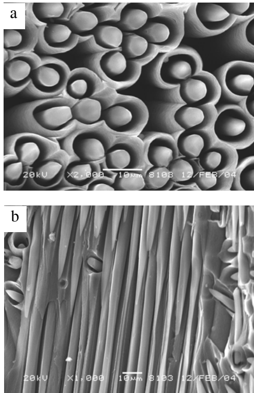
Figure (3) : Ablation morphologies of sample A.
