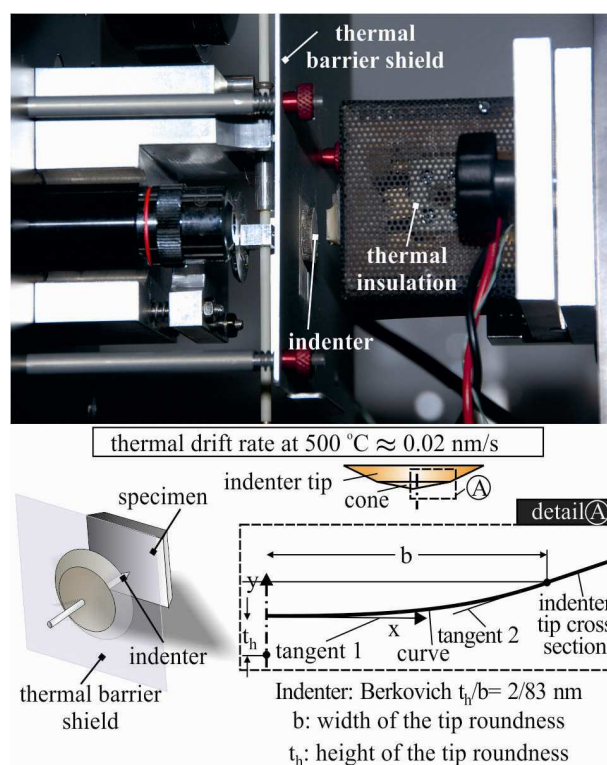
Fig. 1. The applied nanoindentation device and description of the indenter tip geometrical deviations.
