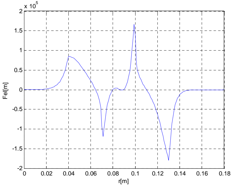
Fig. 7 – The electromagnetic force in the channel.
