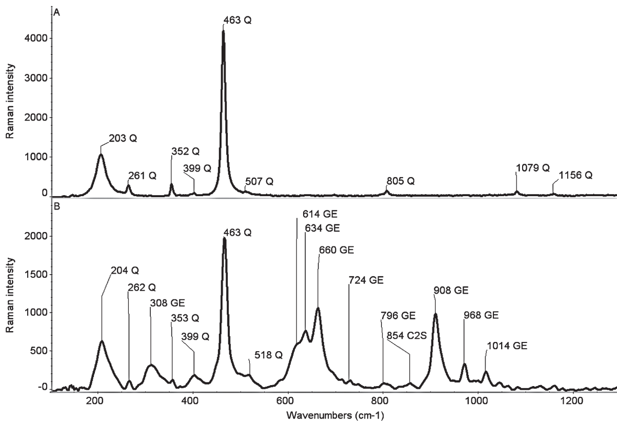
Figure 4. Raman spectra of the fired concrete (A - dark particle in the crack, B - white particle in the crack).
