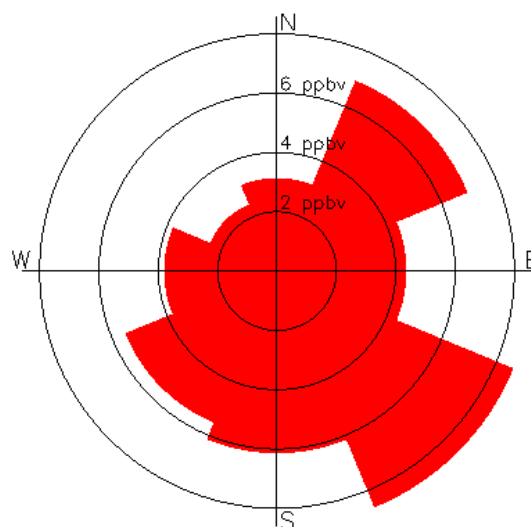
Fig. 7. Average surface \text{NO}_2 mixing ratio during CINDI as a function of wind direction. Included are data between 06:00 and 18:00 UTC and with wind speed exceeding 1.5 \text{ m s}^{-1} .
