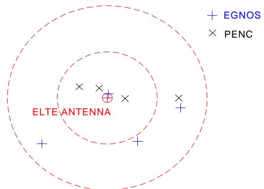
Fig. 7. Test measurements at ELTE Roof Antenna.
