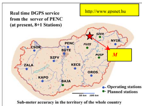
Fig. 1. The distribution of active GPS network.
