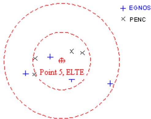
Fig. 6. Test measurements at Point 5 of ELTE site.
