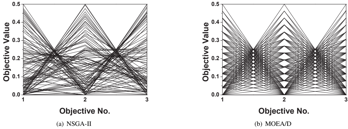
Fig. 11. The corresponding parallel coordinates plots of the solution sets in Figure 10.
