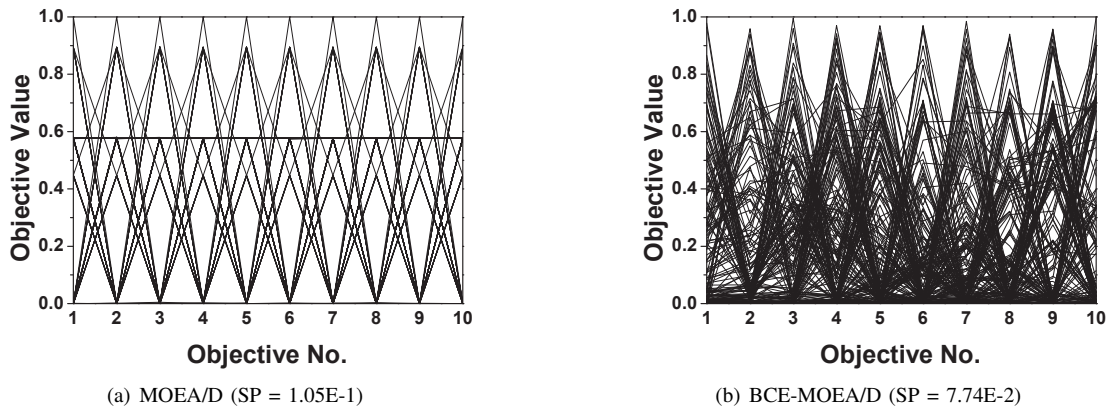
Fig. 13. The solution sets obtained by MOEA/D and BCE-MOEA/D on the 10-objective DTLZ2, and their evaluation results on the uniformity metric SP (the smaller the better).
