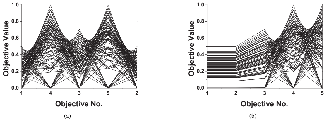
Fig. 21. The solution set of SPEA2+SDE on the 5-objective DTLZ5(I,M) where I = 3 , shown by different order of objectives in parallel coordinates.
