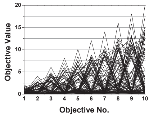
(b) GrEA ( GD^+ = 6.32E-2 )
