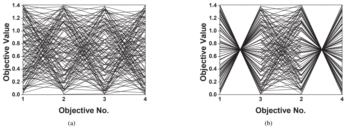
Fig. 22. The solution set of SPEA2+SDE on the 4-objective ML-DMP, shown by different order of objectives in parallel coordinates.
