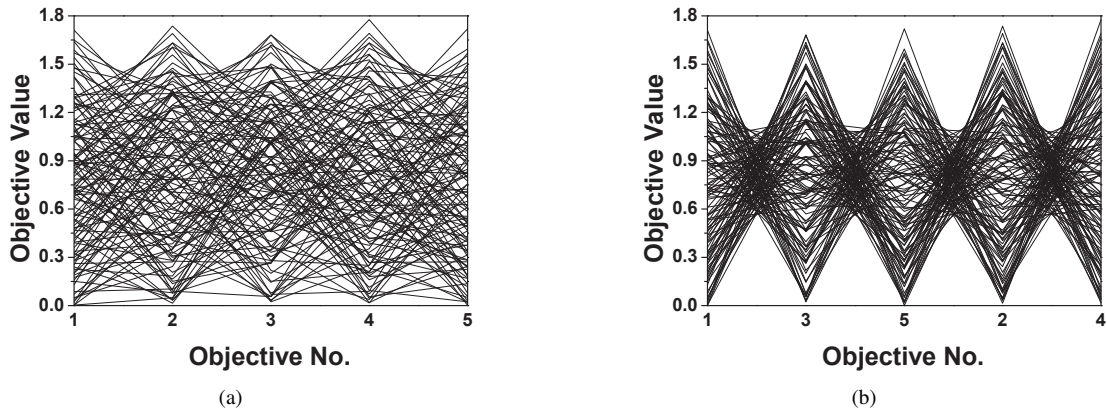
Fig. 20. The solution set of SPEA2+SDE on the 5-objective ML-DMP, shown by different order of objectives in parallel coordinates.
