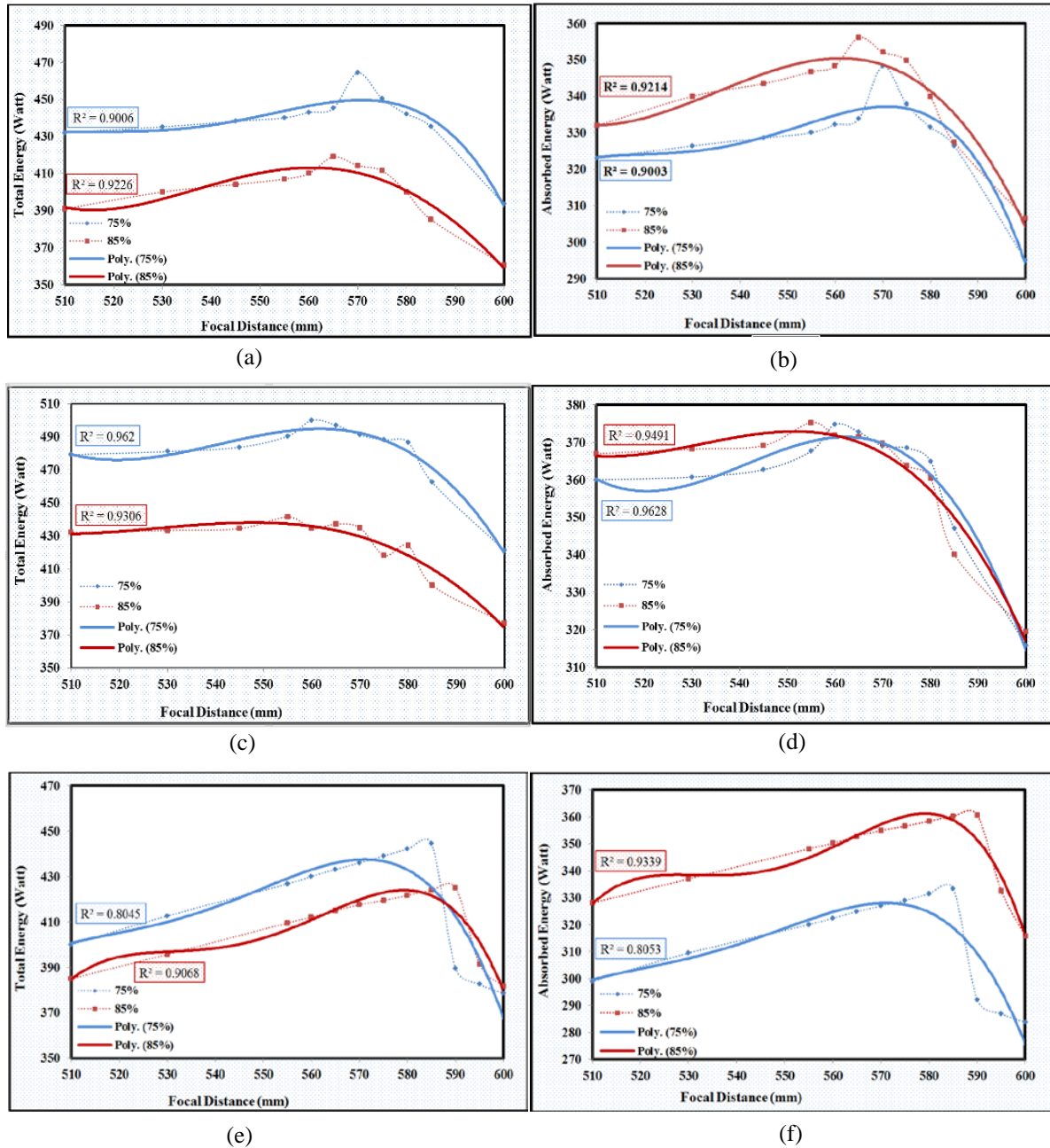
Fig. 15. Total and absorbed energy for at different receiver positions falls on; the spherical shape (a & b), the conical shape (c & d) and the cylindrical (e & f) shape.
