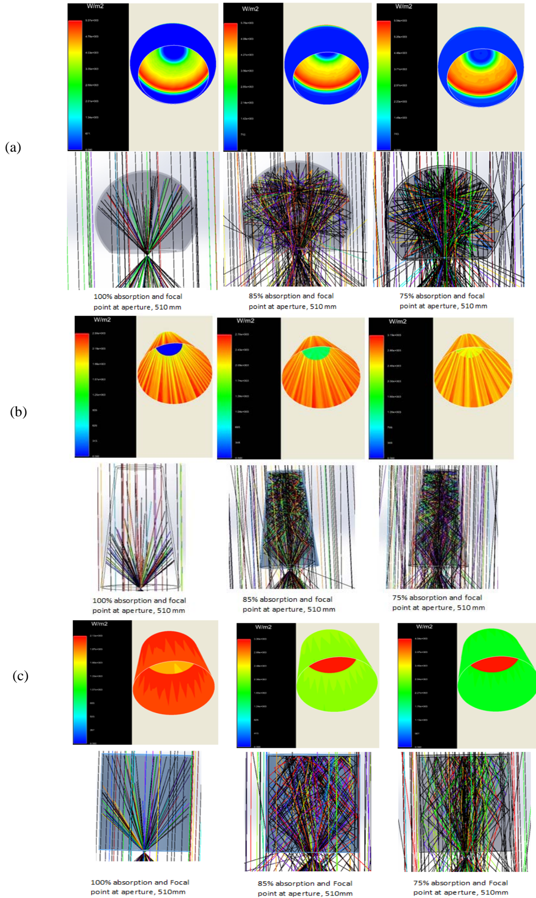
Fig. 10. The effect of absorption ratio on the rays and flux distribution of (a) Spherical shape, (b) Conical shape and (c) Cylindrical shape.
