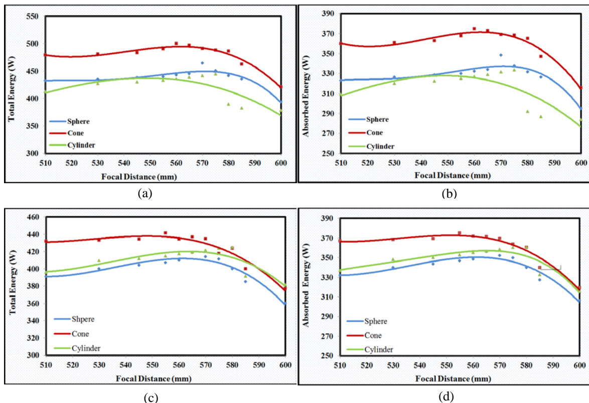
Fig. 16. Total and absorbed energy for the three cavity receivers at different receiver positions and absorption ratios of; 75% (a & b) and 85% (c & d).
