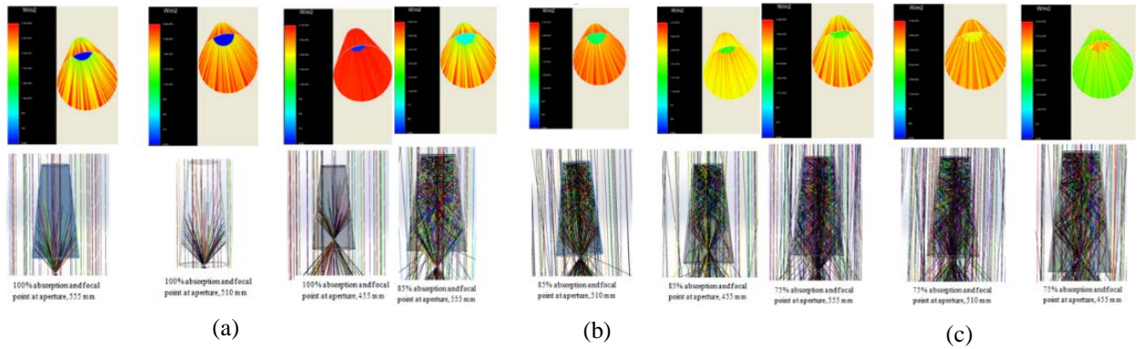
Fig. 12. The effect of receiver position on the rays and flux distributions for; (a) 100%, (b) 85% and (c) 75% absorption ratios.
