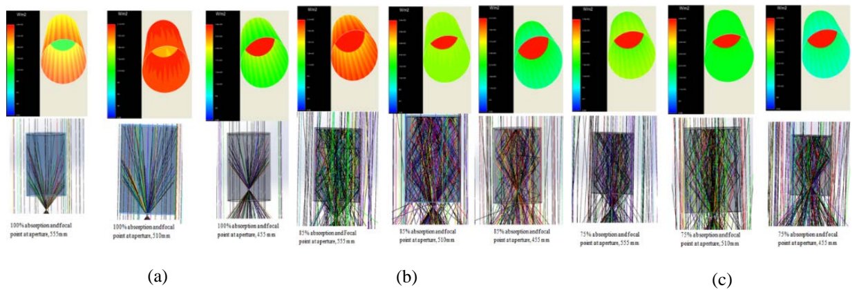
Fig. 13. The effect of receiver position on the rays and flux distributions for; (a) 100%, (b) 85% and (c) 75% absorption ratios.
