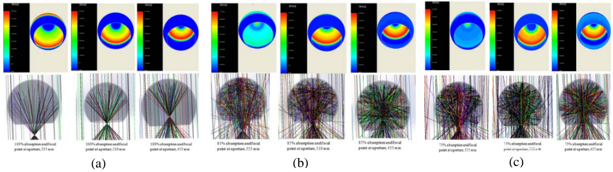
Fig. 11. The effect of receiver position on the rays and flux distributions for; (a) 100%, (b) 85% and (c) 75% absorption ratios.
