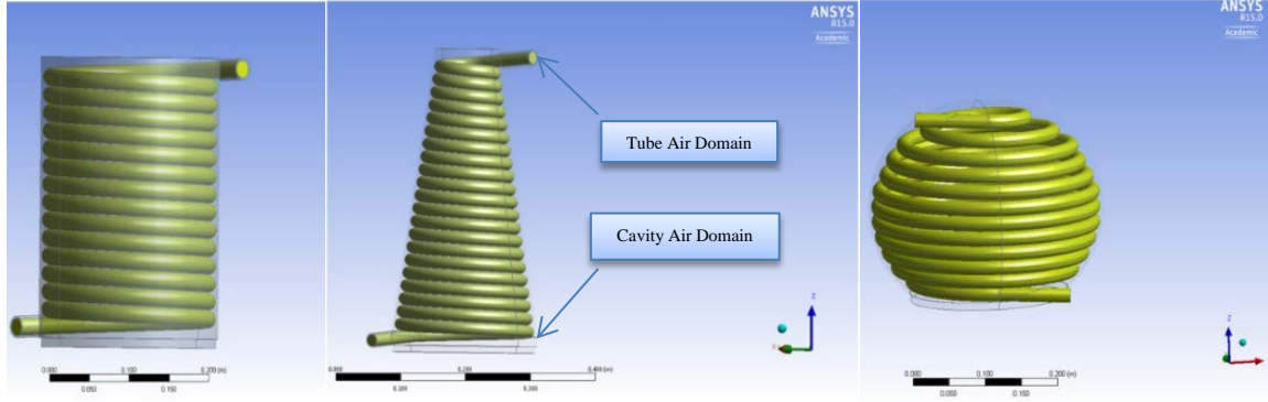
Fig.7. The three shapes of receiver modelled in ANSYS® modular.
