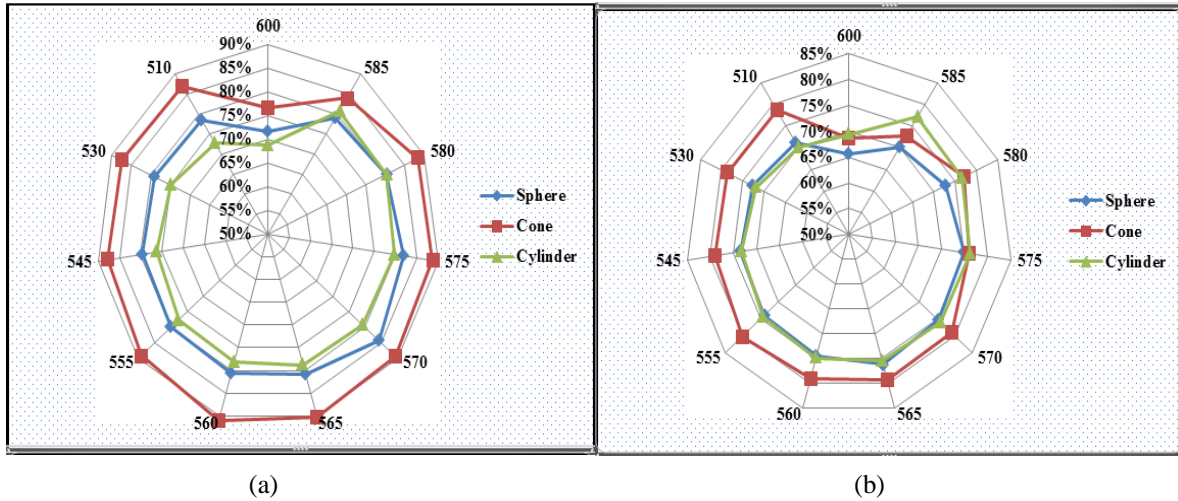
Fig. 17. Optical efficiency for the three cavity receivers at different receiver positions (mm) and absorption ratios of; (a) 75% and (b) 85%.
