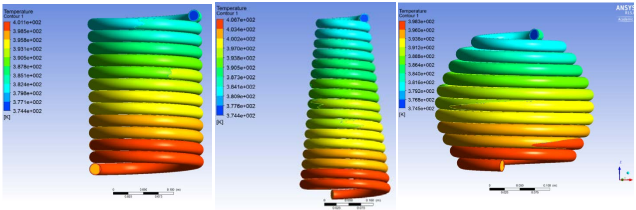
Fig. 19. Temperature distribution for the three receivers.
