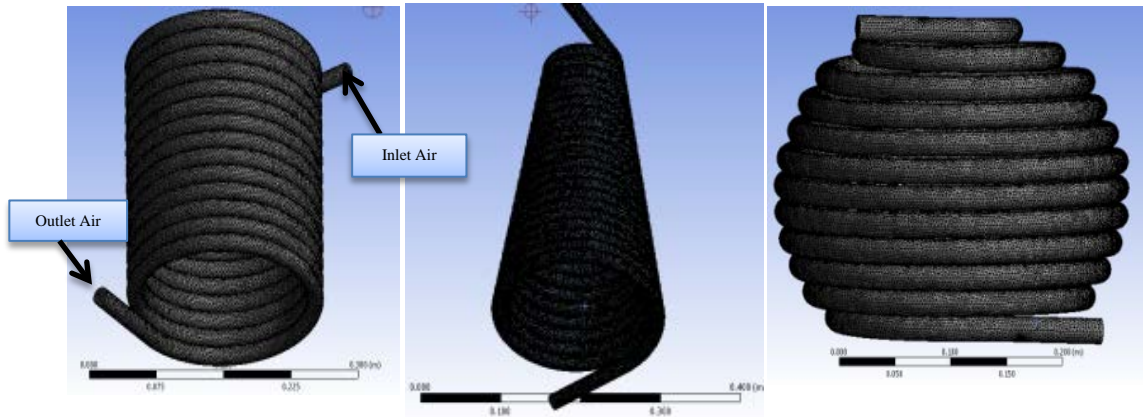
Fig. 8. 3-D Tetrahedral mesh for helical tube of the three receivers.
