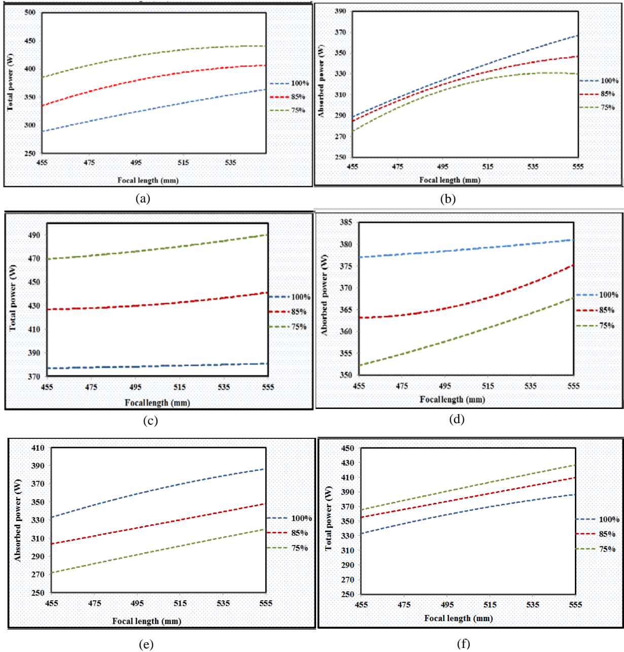
Fig. 14. Total and absorbed energy for the three mentioned positions falls on; the spherical shape (a & b), the conical shape (c & d) and the cylindrical shape (e & f).
