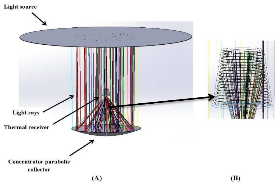
Fig. 5. OptisWorks ® simulation (A): Parabolic concentrator with receiver. (B) Conical receiver.
