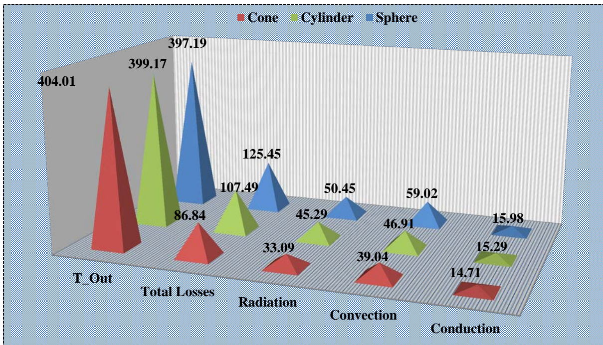
Fig. 20. Conductive, convective, radiative, total heat losses (watt) and outlet temperature of air (K) for the three shapes.
