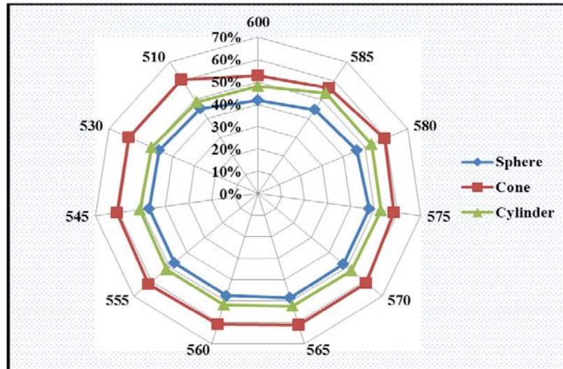
Fig. 21. Combined, optical and thermal efficiency, for the three cavity receivers at different receiver positions (mm) and absorption ratio of 85%.
