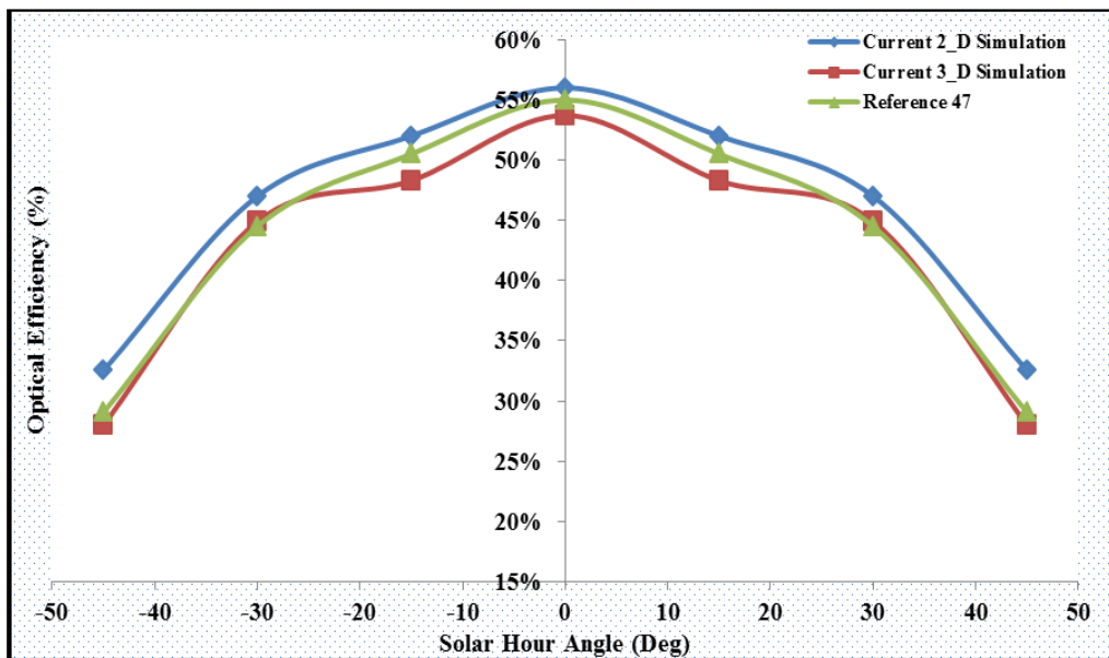
Fig. 6. Comparison the optical efficiency of the current study and reference [47].
