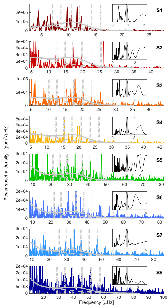
Figure 2. Solar-like oscillation spectra of eight K giants observed by K2. The bottom star is in the RHB. Stars (from top to bottom) are ordered by increasing \nu_{\max} . Vertical lines show the position of radial (dashed lines) and quadrupole (dash-dotted lines) oscillation frequencies as expected by the pattern of oscillation modes in red-giant stars described in Mosser et al. (2011). The expected granulation power and the combined granulation and oscillation power is represented by dashed and solid thick lines. The insets show the power spectrum of the power spectrum (PSPS) of each star, computed from the region around \nu_{\max} . In each PSPS the prominent peak at \Delta\nu/2 (vertical gray line) is the detected signature of the near-regular spacing of oscillation peaks in the frequency spectrum.
