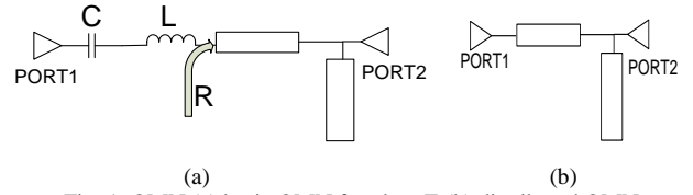
Fig. 1. OMN (a) basic OMN for class-E (b) distributed OMN
