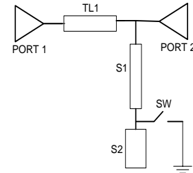
Fig. 6. Switched-band OMN
