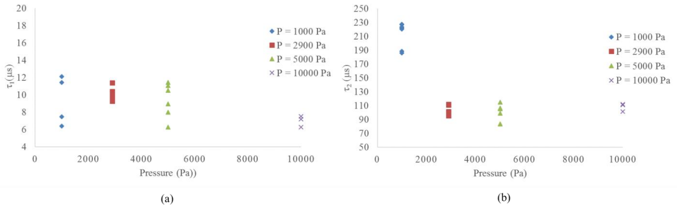
Figure 4(a) rapid decay time constant at 298 \text{ K} , (b) slow decay time constant at 298 \text{ K}
