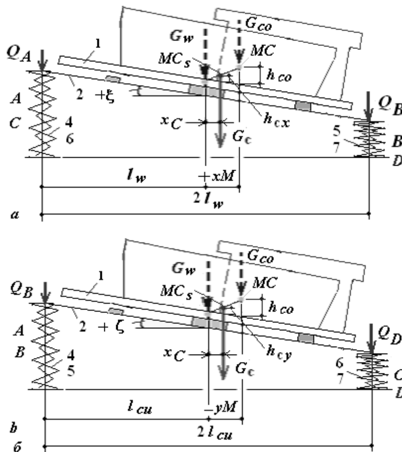
Fig. 2. Redistribution of carriage underframe pressure force on bogie spring sets: a – in cargo displacement lengthwise the wagon; b – in cargo displacement crosswise the wagon
