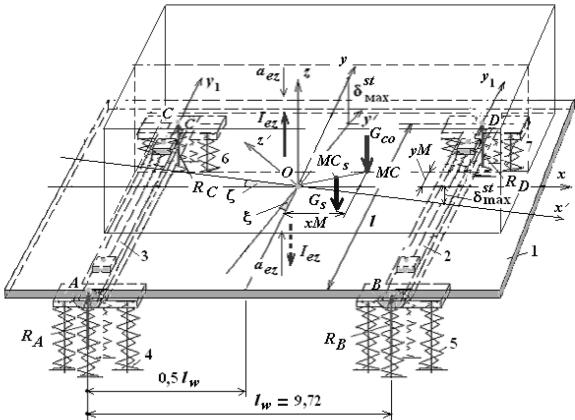
Fig. 1. Determination of a bogie spring set response: 1 – carriage underframe, 2 и 3 – bolsters , 4 – 7 – spring sets
