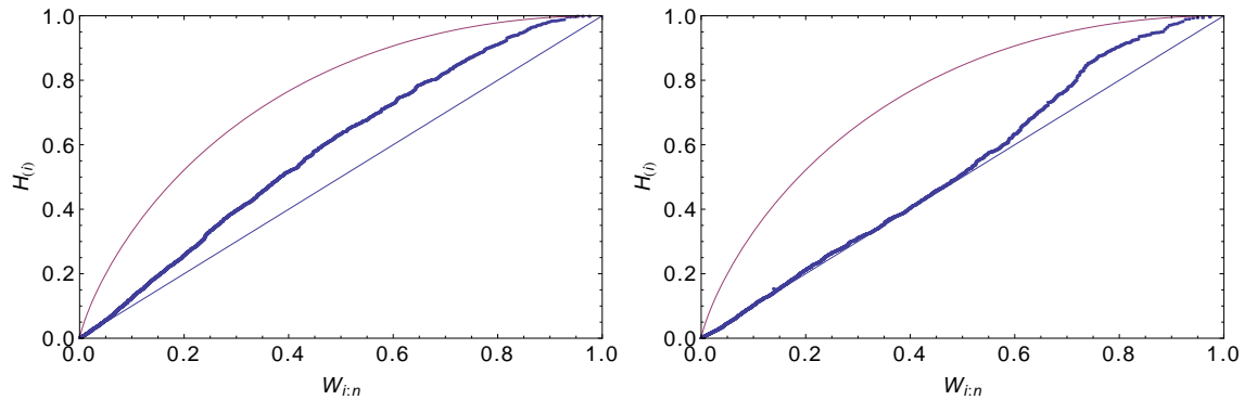
Fig. 6. K-plot of the observed rainfall time series at station Garmisch-Partenkirchen (Germany) before ARMA-GARCH transformation (left), and after ARMA-GARCH transformation (right). Superimposed on the graph are a straight line (blue) corresponding to the case of independence and a curve corresponding to perfect positive dependence (red).
