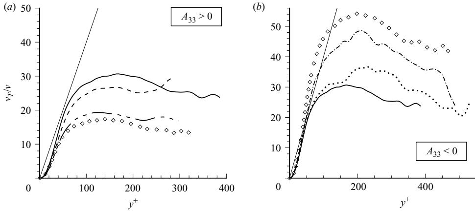
FIGURE 5. Inner scaling of eddy viscosity v_\tau = -\overline{u'v'}/(\partial\overline{u}/\partial y) for ZPG lateral (a) divergence and (b) convergence at At=0.38 : ----, Case SD; - - - - - , Case FD; ······, Case SC; — · — ·, Case FC; ———, unstrained initial condition ( At=0 ); \diamond , rapid-distortion limit, v_\tau(t, y_w)/v_\tau(0, y_w) = \exp(-(3/2)A_{33}t) , with y^+(t)/y^+(0) = \exp(-(1/2)A_{33}t) . Thin solid straight line is 0.4 y^+ .
