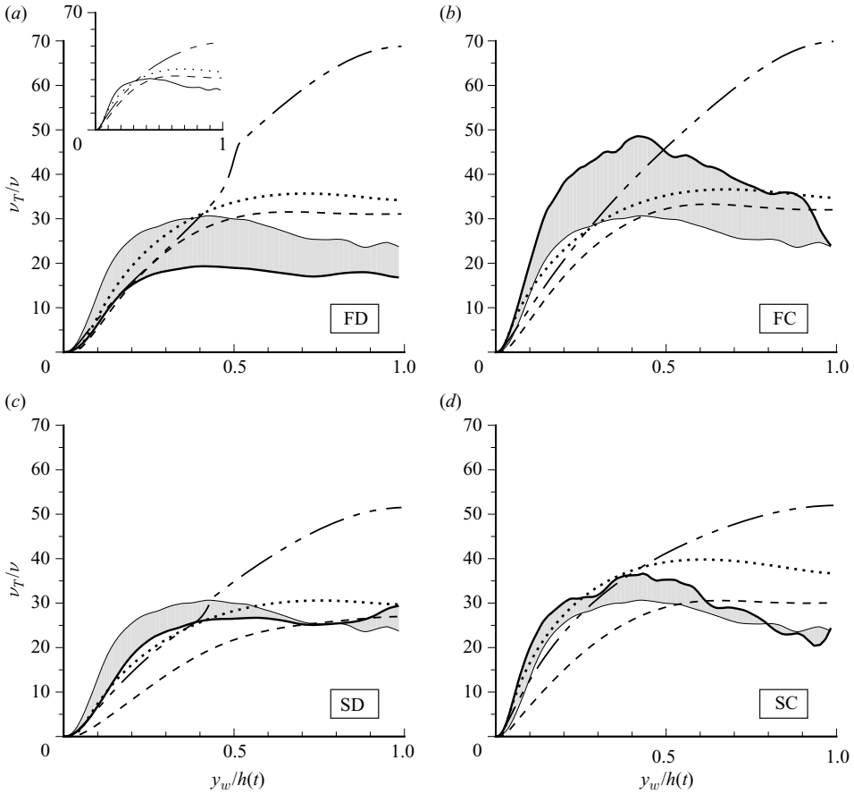
FIGURE 16. DNS and model predictions of eddy viscosity \nu_T at At=0.38 : —, -\overline{u'v'}/(\partial\bar{u}/\partial y) from DNS; ·····, Spalart–Allmaras; ———, Menter SST; -·-·-, Wilcox Stress- \omega . Shaded regions indicate strain-induced departure of DNS from unstrained initial conditions, denoted by thin-solid (—) curve. Inset plot in (a) illustrates DNS and model profiles at At=0 .
