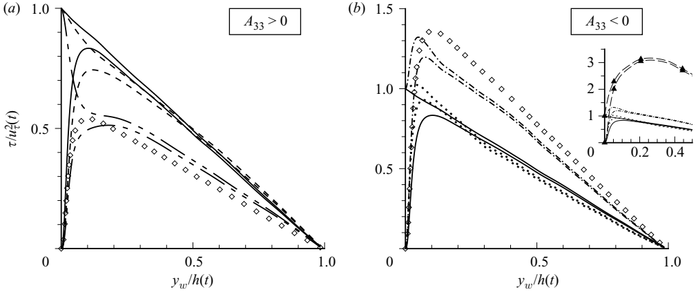
FIGURE 4. Total and Reynolds shear stress in local u_\tau(t) scaling for ZPG lateral (a) divergence and (b) convergence at At=0.38 : ----, Case SD; - · - · -, Case FD; · · · · ·, Case SC; — — —, Case FC; ———, unstrained initial condition ( At=0 ); \blacktriangle , APG strain at A_{22}t=0.365 from Coleman et al. (2003) (inset in (b) only); \diamond , rapid-distortion limit, -\overline{u'v'}(t, y_w) = -\overline{u'v'}(0, y_w) \exp(-(1/2)A_{33}t) , normalized by u_\tau^2 at At=0.38 from Cases (a) FD and (b) FC.
