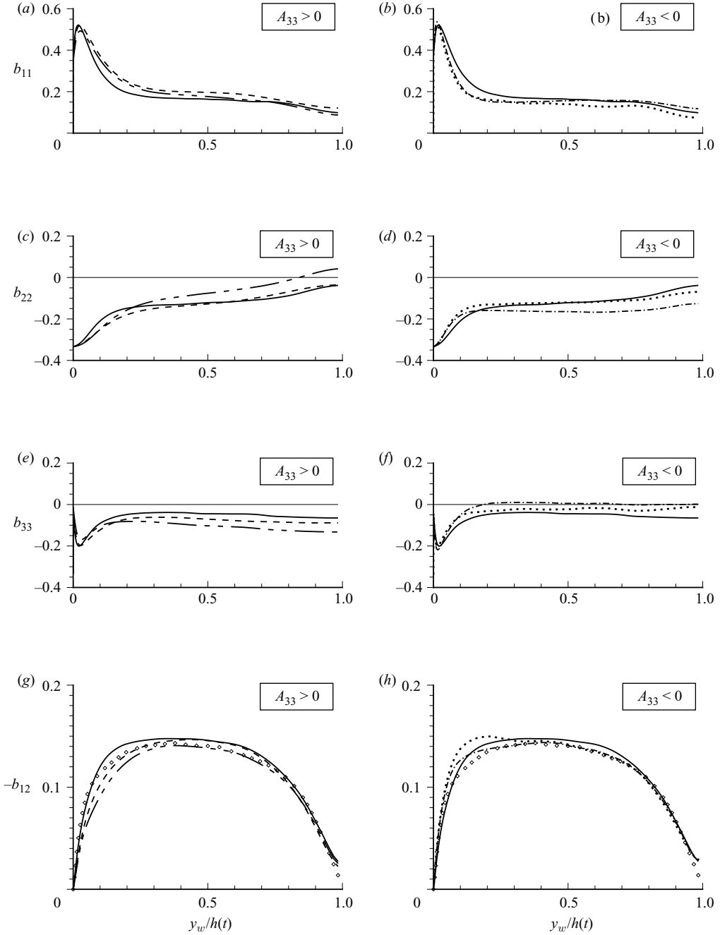
FIGURE 11. Components of Reynolds-stress anisotropy tensor \mathbf{b}_{ij} = \overline{u'_i u'_j} / q^2 - (1/3)\delta_{ij} for ZPG lateral (a, c, e, g) divergence and (b, d, f, h) convergence at At = 0.38 : ----, Case SD; - · - ·, Case FD; ·····, Case SC; —, unstrained initial condition ( At = 0 ); ◇, APG strain at A_{22}t = 0.365 from Coleman et al. (2003) (g and h only).
