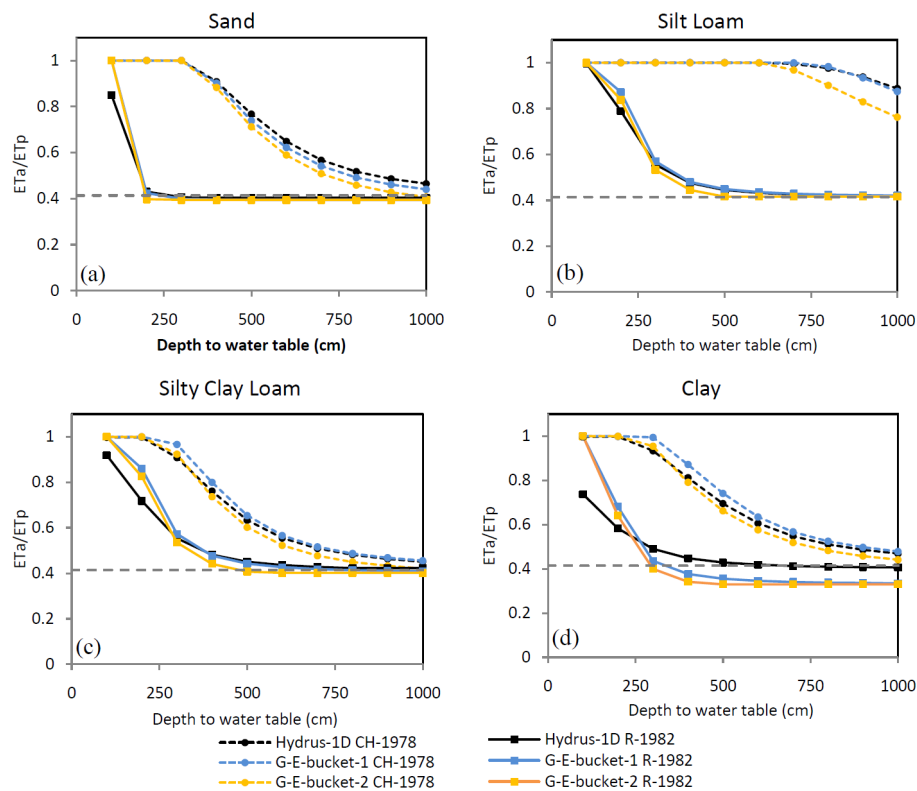
Fig. 6. Same as in Fig. 4, except for daily Hydrus-1D (black) and G-E-bucket model (1-blue, 2-yellow) 10-year simulations (see Table 3). The node spacing in the Hydrus-1D simulation is 1.5 cm, and ET_p is calculated from the Priestley-Taylor relationship.
