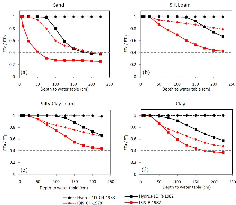
Fig. 5. Same as in Fig. 4, except for hourly Hydrus-1D (black) and IBIS (red) 10-year simulations (see Table 3). The node spacing in all simulations is 2.5 cm, and ET_p is calculated based on ET_a from the “saturated” IBIS run.
