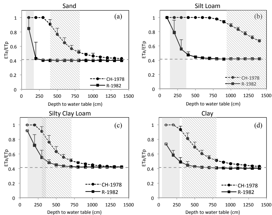
Fig. 4. Long-term mean annual ET_a/ET_p versus water table depth, based on the daily Hydrus-1D 10-year simulations (see Table 3). Shown are model results for (a) sand, (b) silt loam, (c) silty clay loam, and (d) clay. Dashed and solid lines indicate model solutions using Clapp and Hornberger (1978) and Rawls et al. (1982) soil parameters, respectively (both with 1.5-cm node spacing). Vertical “error bars” represent solutions using 30-cm node spacing, while empty squares or circles indicate solutions that did not converge using a 30-cm nodal distance. The horizontal, dashed line (in grey) indicates the 10-year mean annual P/ET_p ratio, where ET_p is calculated from the Priestley-Taylor relationship. Gray shaded and hatched areas represent approximate critical zones for R-1982 and CH-1978 soil parameters, respectively.
