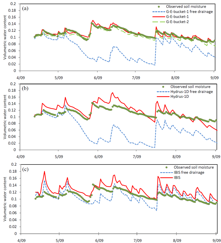
Fig. 3. Observed and simulated depth-averaged soil moisture (i.e., volumetric water content down to 50 cm) for the (a) two G-E bucket models, (b) Hydrus-1D model, and (c) IBIS model during the 2009 model evaluation period (see Table 3). Simulation results using free drainage as the lower boundary condition are represented by blue dashed lines. Green dots show the daily mean soil moisture observations from the field site.
