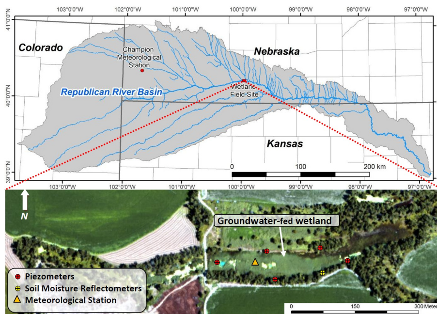
Fig. 1. Map showing the location of the piezometers, soil moisture reflectometers, and meteorological station at the wetland field site in the Republican River basin, as well as the location of the HPRCC climate station in Champion, Nebraska.
