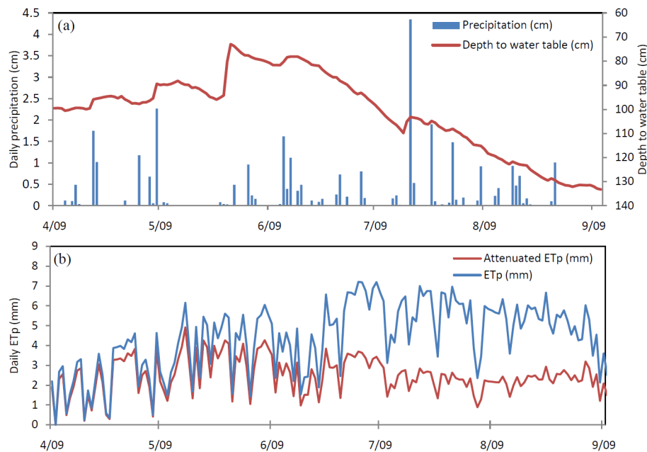
Fig. 2. (a) Observed daily precipitation and water table depth for the field site in south-central Nebraska during the 2009 growing season. (b) Daily ET_p (calculated from the Priestley-Taylor equation) and “attenuated ET_p ” for the understory vegetation (based on LAI-reduced net radiation due to overstory vegetation).
