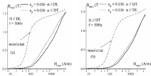
Fig.5: The magnetization curves of the alloy Fe-3%Si NO measured in the rolling direction and in the cross section direction(b) for a plastic deformation around 3,6%, the solicitation parallel with the measurement direction and in a perpendicular direction. Comparison with the not out of shape state.
