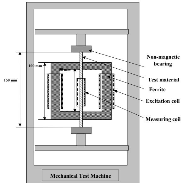
Fig.6: The general scheme of the magnetic characterization device during a uniaxial traction solicitation
