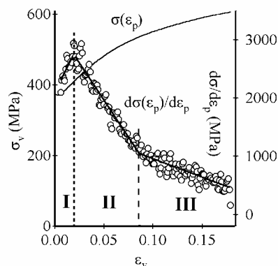
Fig. 1: The traction curve (depending on the plastic deformation and the cold hammering coefficient for the alloy Fe-3%Si and the deformation speed around 1,33 \cdot 10^{-3} \text{s}^{-1} (Hubert,1998).
