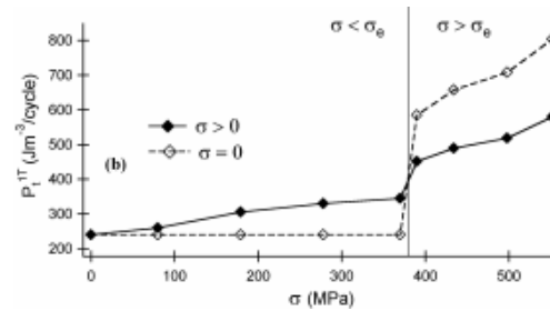
Fig.9: The evolution of the maximum induction B_{max} at 1000 A/m (a) and total losses of energy P_t at IT (b) for a test specimen Fe-3%Si NO during a loading-unloading solicitation in uniaxial traction (magnetic excitation frequency 50 Hz)
