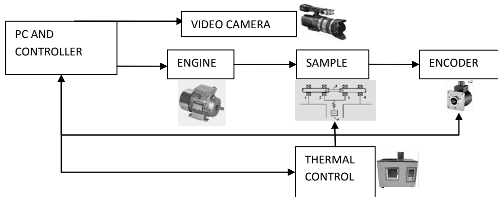
Figure 8: Functional Scheme.
