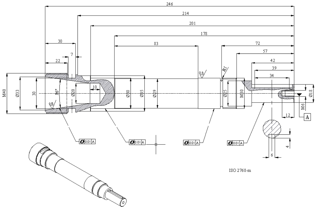
Figure 4: Driven shaft.
