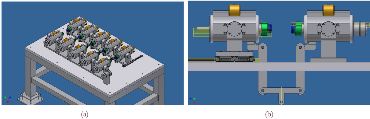
Figure 5: Spindles group: a) total view; b) load system details.
