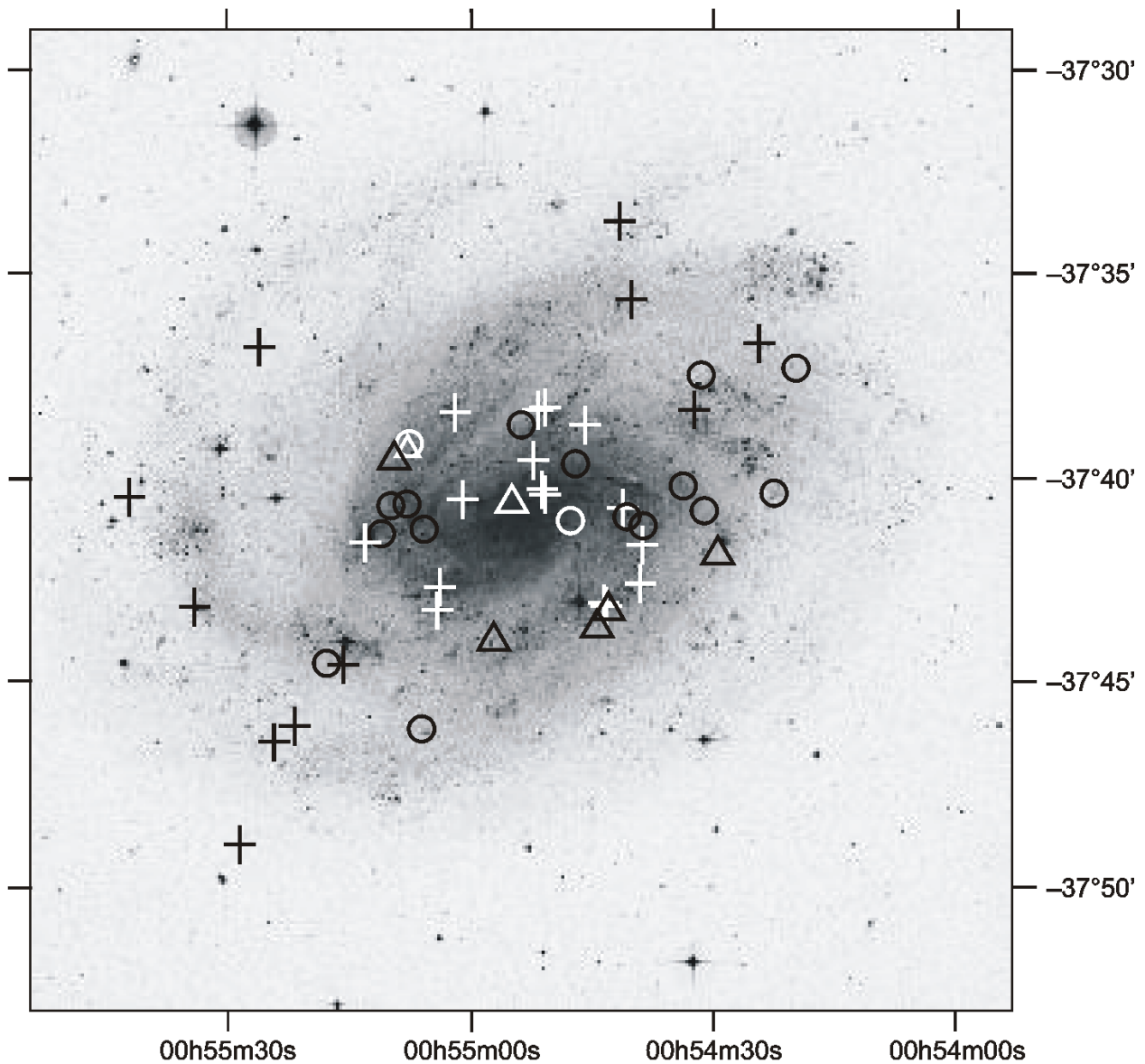
Fig. 1. A DSS image of NGC 300 with the positions (in J2000.0 coordinates) indicated of the 51 SNRs and candidate SNRs considered by the present study. Radio sources (SNRs and SNR candidates only) from P04 are shown with crosses. Optical candidates with line ratios measured with long-slit spectra (from BL97) are shown as circles and optical candidates with line ratios measured by interference filters (BL97) are shown with triangles. Symbols are black or white only for increased contrast. (Figure originally published in MWF11. Southern sky DSS image, courtesy of Royal Observatory Edinburgh, Anglo-Australian Observatory, California Institute of Technology.)
