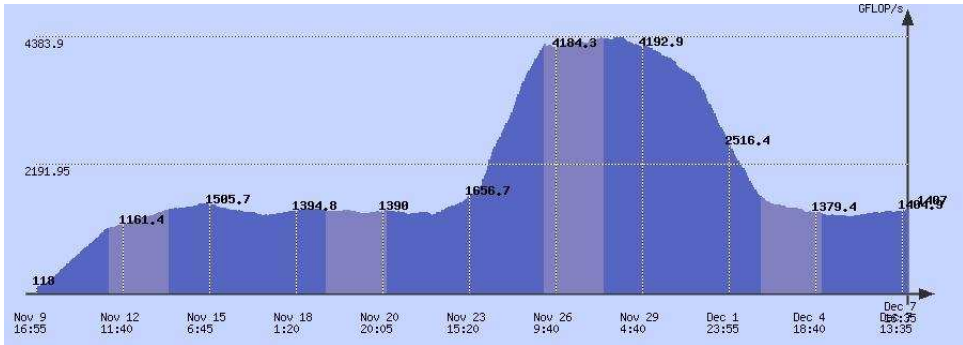
Figure 4. The dynamics of real performance of SAT@home (GFLOPs)
