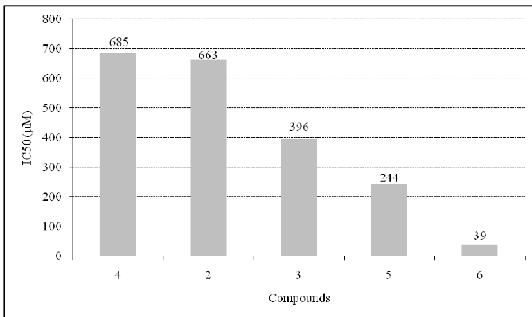
Figure 2. IC 50 (µM) Values of isolated compounds for lipid peroxidation inhibition. Rosmarinic acid (2); Luteolin 7- O -(6''-feruloyl)-β-glucopyranoside (3); Luteolin (4); Luteolin 5- O -β-glucopyranoside (5); Luteolin 7- O -β-glucuronide (6)
