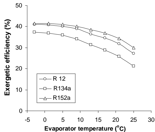
Fig. 4. Variation of Exergetic Efficiency with Evaporator Temperature.
