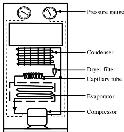
Fig. 2. Schematic Diagram of Experimental Refrigerator.
