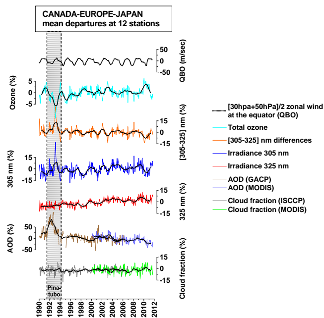
Fig. 1. Changes in (%) in total ozone, UV irradiances at 305 and 325 nm, AOD at 550 nm and cloud fraction averaged over 12 stations located between 25° N and 60° N. The third time series shows the long-term variability of the difference (in %) between 305 nm and 325 nm solar spectral irradiance. Solid black curves are 12-month running means.
