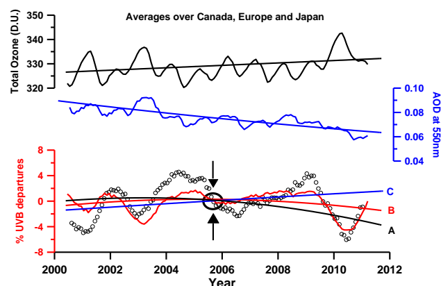
Fig. 4. Upper part: total ozone (12 month running mean) from ground-based measurements at 12 stations, Middle: average AOD from MODIS/Terra (12 month running mean) over the 12 stations. Lower part: 305 nm irradiance departures (red) calculated with the RT model, and open circles are observed 305 nm solar irradiances. Curves A, B, C are 2nd deg. polynomial fit of the calculated contribution of ozone (A), aerosol (C) and ozone and aerosol together (B) to the 305 nm irradiance variation.
