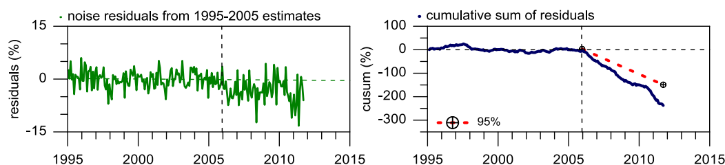
Fig. 3. White noise residuals (left panels) and their CUSUMs ( \varepsilon_t , right panels) for all stations average. The red dotted line indicates the negative part of the 95 % confidence envelope of departures from natural variability and model uncertainty.
