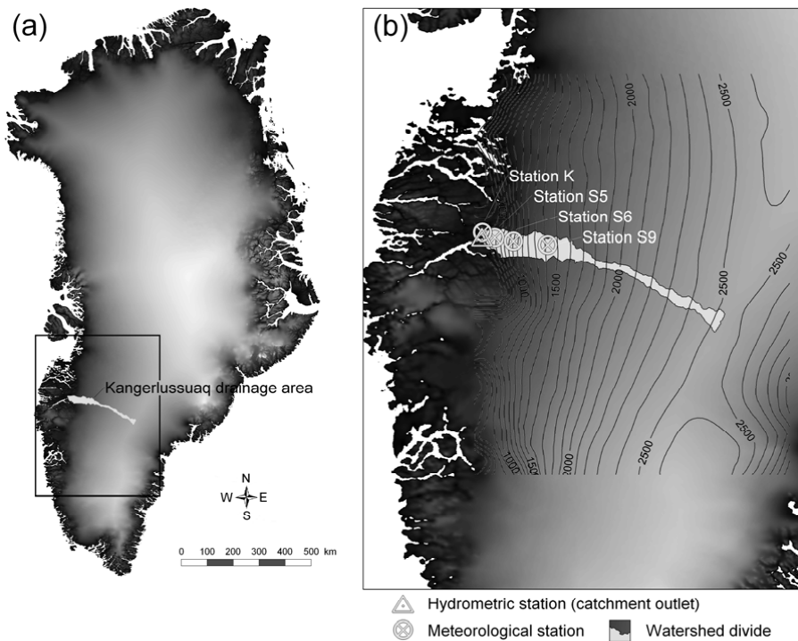
Fig. 1. (a) Greenland including the Kangerlussuaq drainage area (6130 km 2 ) in West Greenland; (b) simulation area with topography (gray shades, and 100-m contour interval), the four meteorological stations: Station K (50 m a.s.l.), S5 (490 m a.s.l.), S6 (1020 m a.s.l.), and S9 (1520 m a.s.l.), the hydrometric station at the catchment outlet, and the catchment watershed divide. The catchment watershed divide was established in River Tools based on the surface DEM by Bamber et al. (2001).
