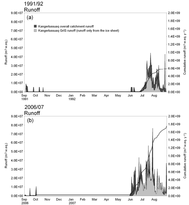
Fig. 4. (a) and (b) Time series of daily modeled runoff for the Kangerlussuaq part of the GrIS and for the Kangerlussuaq drainage area for 1991/1992 (the year with the lowest annual cumulative runoff) and 2006/2007 (highest cumulative runoff). The period from September through August follows the fixed GrIS mass-balance year.
