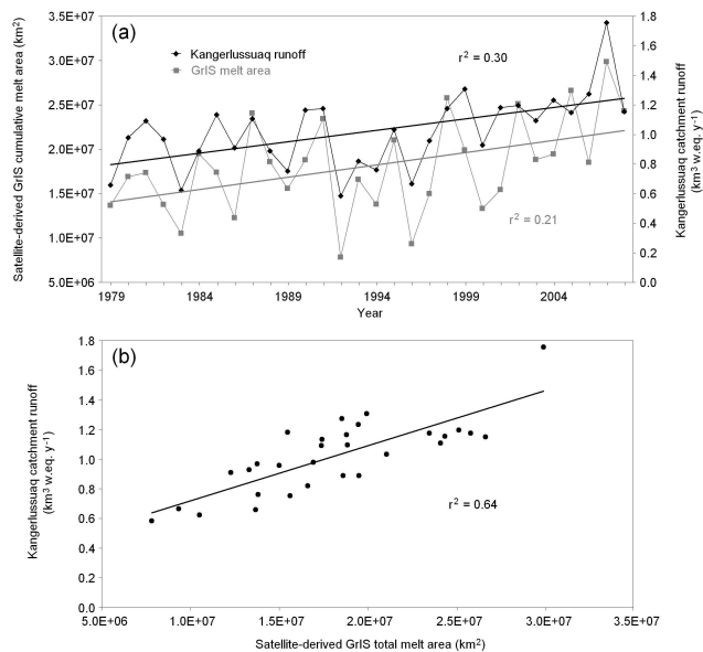
Fig. 5. (a) Time series of Kangerlussuaq simulated runoff and passive microwave satellite-derived GrIS cumulative melt extent area (satellite data provided by CIRES, University of Colorado at Boulder) for 1979 through 2008; and (b) relation between satellite-derived GrIS cumulative melt area and Kangerlussuaq catchment runoff. Without the extreme 2006/2007 anomaly the r^2 was 0.57.
