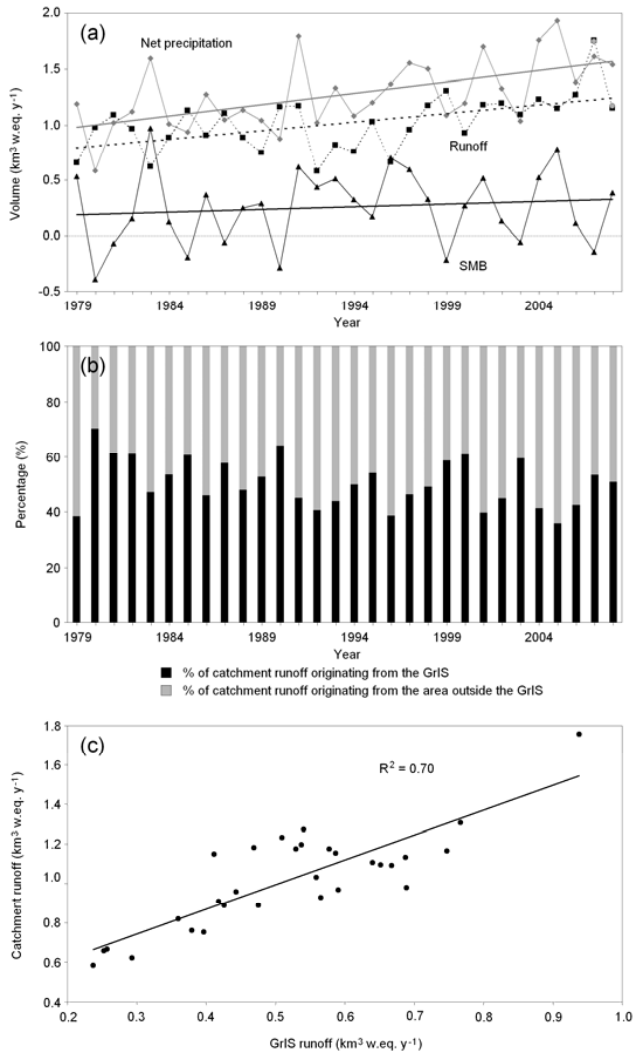
Fig. 3. (a) Kangerlussuaq net precipitation, runoff, and change in storage ( \Delta S ; SMB) series for 1978/1979 through 2007/2008. For 2007 and 2008, the observed June through August runoff is further illustrated based on data from Mernild et al. (2009); (b) percentage of catchment runoff originating from the GrIS and the proglacier landscape (to get the runoff contribution from the proglacier landscape, the GrIS runoff was subtracted from the overall catchment runoff); and (c) relationship between GrIS runoff and Kangerlussuaq catchment runoff.
