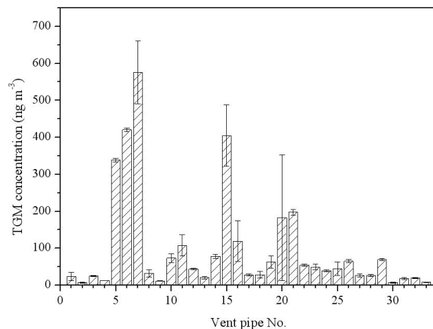
Fig. 8. Average TGM concentrations in the LFG at G-Y (vent pipe No. 1–27) and J-K (vent pipe No. 28–33) landfill, the error bars denote \pm 1 SD in the measured values.
