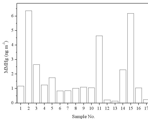
Fig. 10. MMHg in the LFG of selected vent pipes at G-Y landfill.
