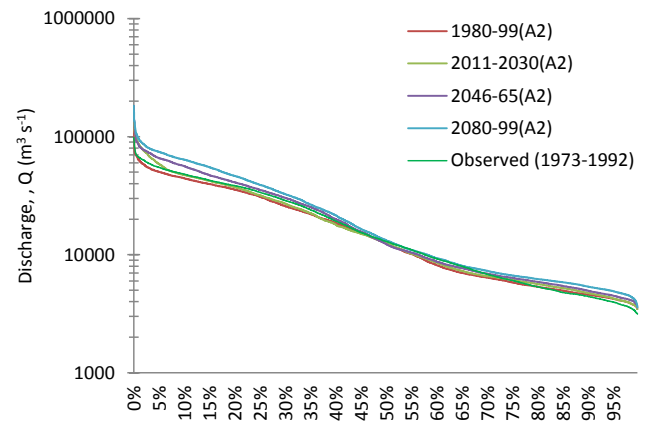
Fig. 6. Flow duration curve for observed and multi-model weighted discharge of A2 scenario of four different time slices.
