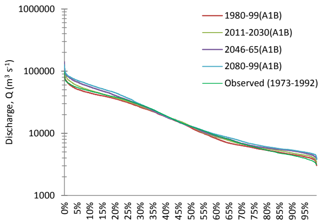
Fig. 5. Flow duration curve for observed and multi-model weighted discharge of A1B scenario of four different time slices.
