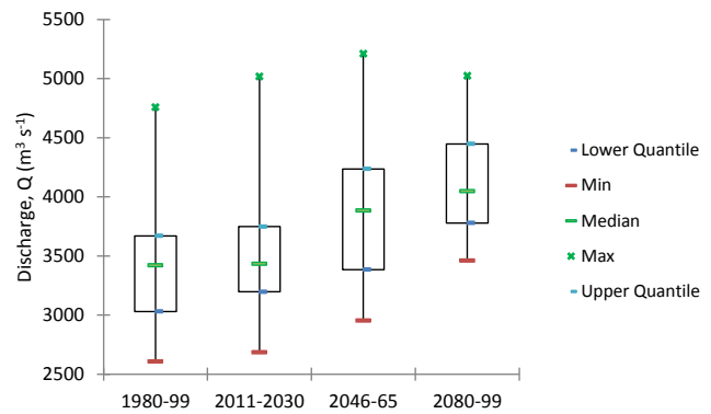
Fig. 8. Box-whisker plot for yearly average 7-day low flow for A1B Scenario of 12 different weighted hydrological model outputs.
