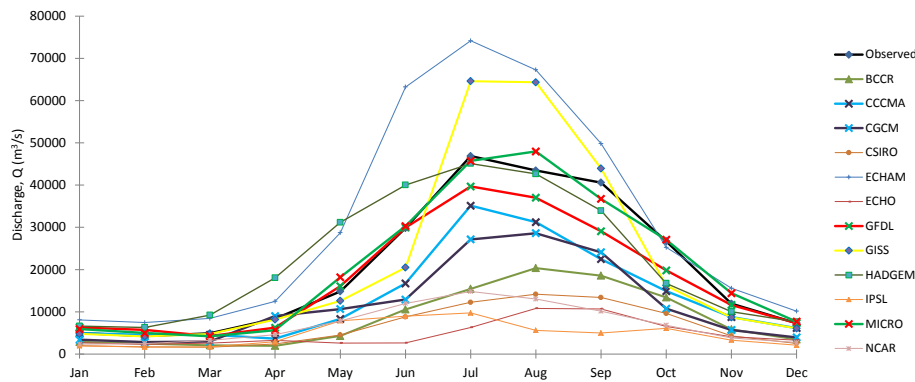
Fig. 2. Comparison of monthly mean discharge as simulated by PCR-GLOBWB with different GCMs as input with that obtained from observed discharge at Bahadurabad station.
