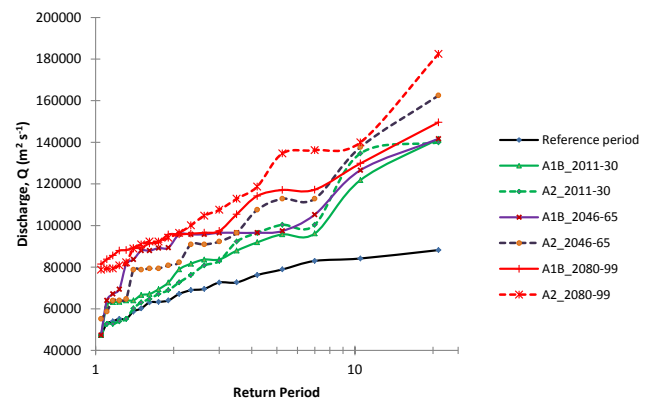
Fig. 9. Annual peak flow for different return periods, time slices and scenario's obtained from a weighted average of extreme value analysis of the 12 model outputs.
