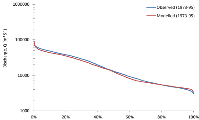
Fig. 3. Comparison of flow duration curve between observed and discharge weighted modelled data for the period 1973–1995.
