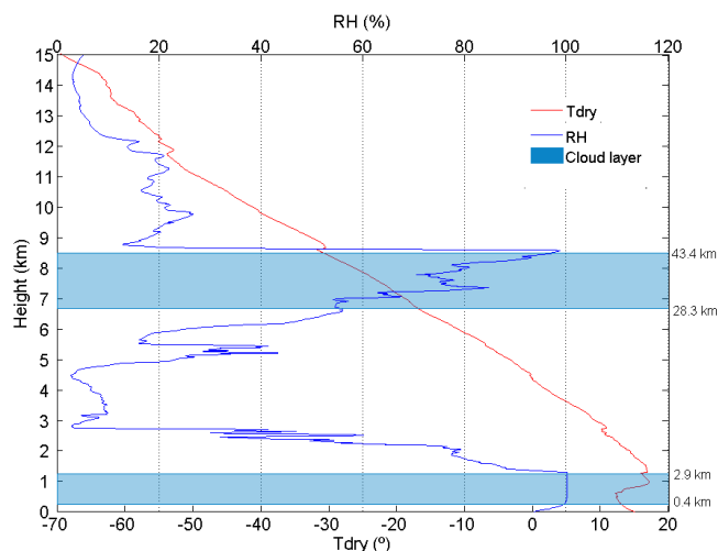
Figure 1. Temperature ( T_{\text{dry}} (°), in red) and relative humidity with respect to water (RH (%), in blue) profiles above ground level from the radiosonde on 5 October 2009 at 23:23 h at SGP. Blue shading represents the cloud layers as detected by ARSCL. The values (on the right) related to every cloud layer boundary indicate the sonde horizontal distance from the ARSCL site in kilometers when it reached those altitudes.
