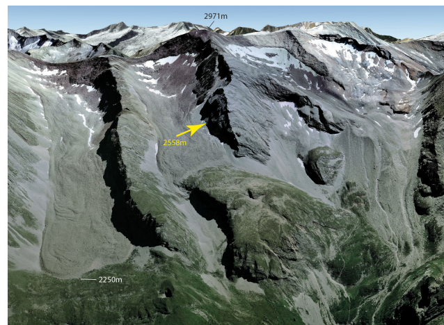
Figure 2. Oblique aerial view of the setting of the MSK Cave (entrance marked by the yellow arrow) at the Tuxer Hauptkamm, Zillertal Alps. Note active rock glaciers occupying the cirques and reaching down to 2250 m in case of the rock glacier in the left cirque. View to the southeast (Google Earth Pro image).
