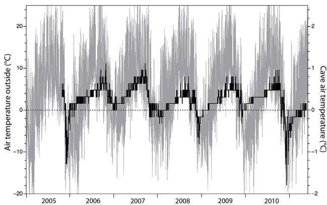
Figure 5. The air temperature near the lower end of MSK Cave (black) mirrors the outside temperature changes (grey) until about November; afterwards the cave air temperature for most of the years is decoupled from the outside air, suggesting that snow clogs the entrance during winter. The outside temperature was recorded at Spannagel Hut located at 2531 m 6.5 km southwest of MSK Cave.
