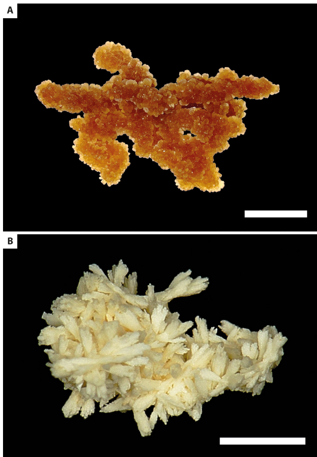
Figure 7. Morphology of cryogenic calcite crystals in normal reflected light. (a) Typical brown crystal aggregate; sample MSK1. Scale bar 3 mm. (b) White crystal aggregate; sample MSK5. Scale bar 1 mm.
