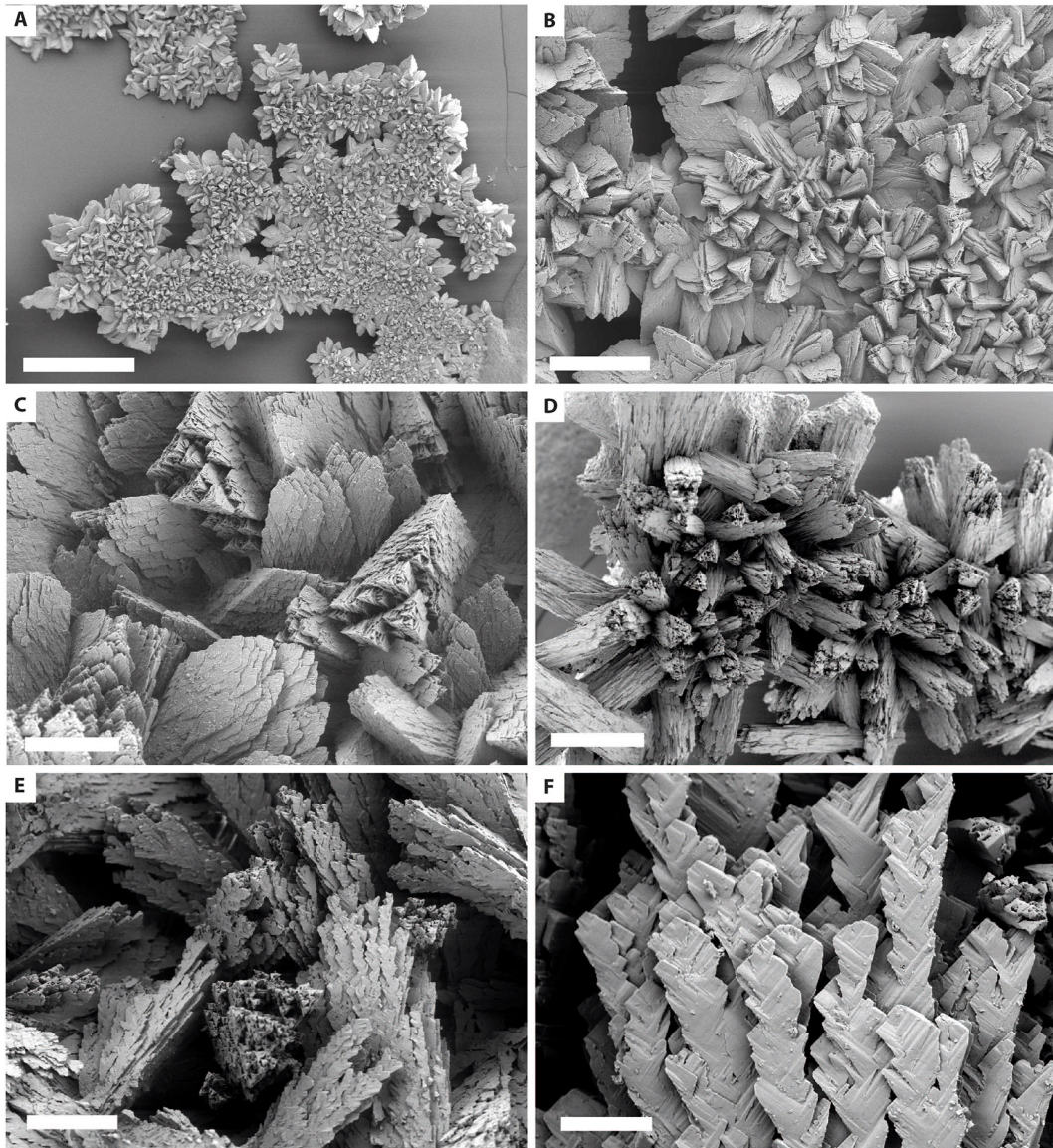
Figure 8. Morphology of cryogenic calcite crystals seen under the FE-SEM. (a) Calcite raft; sample MSK5B. Scale bar 1 mm. (b) Close-up of (a). Scale bar 0.2 mm. (c) Stepped faces on individual rhombohedral crystals; sample MSK6B. Scale bar 0.1 mm. (d) White crystal aggregate; sample MSK3W. Scale bar 0.2 mm. (e) Details of white crystal morphology; sample MSK5W. Scale bar 0.1 mm. (f) Close-up of (e), revealing chevron-type crystal habits. Scale bar 0.02 mm.
