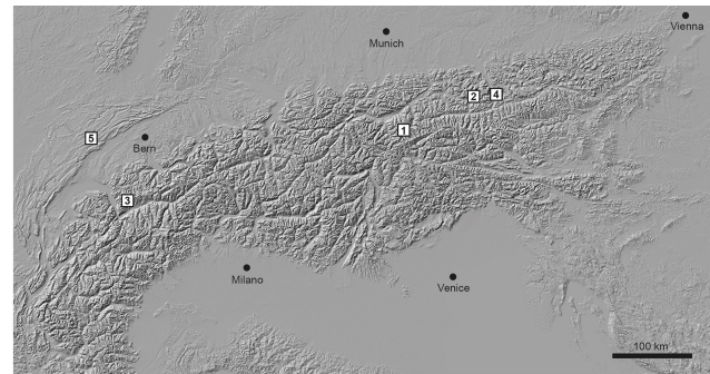
Figure 1. Elevation map of the Alps showing the currently known locations of CCC_{\text{coarse}} (1: MSK Cave (this study); 2: Glaseis Cave; 3: Leclanché Cave) and CCC_{\text{fine}} (4: Eisriesenwelt; 5: Monlesi Cave; as well as also in Leclanché Cave, no. 3).
