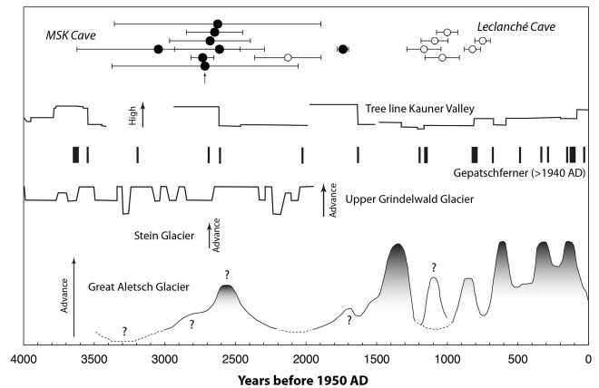
Figure 11. ^{230}\text{Th} dates of CCC_{\text{coarse}} from MSK Cave (filled circles) and the west-Alpine Leclanché Cave (open circles; Luetscher et al., 2013) compared to changes in the elevation of the tree line in the central-Alpine Kauner Valley (Nicolussi et al., 2005), advances of the east-Alpine Gepatsch Glacier beyond the extent of the 1940 AD glacier size (Nicolussi and Patzelt, 2001), a speleothem-based record of the ice surface elevation of the Upper Grindelwald Glacier (Luetscher et al., 2011), ^{10}\text{Be} -dated evidence of a marked advance of Stein Glacier, Switzerland (Schimmelpfennig et al., 2014), and a semicontinuous glacier-length record of the Great Aletsch Glacier in the Western Alps (Holzhauser et al., 2005) for the last four millennia. The only date of the white crystal fraction from MSK Cave is marked by a small vertical arrow.
