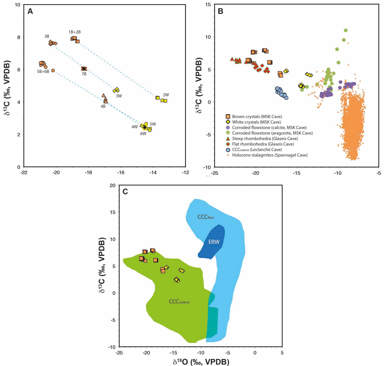
Figure 10. Stable isotopic composition of CCC coarse samples from the two chambers in MSK Cave. Note different but equidistant scales on all three diagrams. (a) Brown (B) and white (W) crystal populations of individual CCC occurrences often show unique isotopic signatures. If both populations are present in one sample (as is the case for samples MSK2, 3, 4, 5 and 6), they define end members of linear relationships whose negative slopes are very similar. (b) Comparison of CCC coarse samples from MSK Cave with CCC coarse samples from Glaseis Cave (Richter et al., 2009), Leclanché Cave (Luetscher et al., 2013), inactive flowstone from the Eiskammer of MSK Cave and Holocene speleothems from nearby Spannagel Cave. The latter data set comprises data from 11 stalagmites, including the COMNISPA2 stack (Fohlmeister et al., 2013). (c) CCC coarse samples from MSK Cave in comparison to published CCC coarse (green) and CCC fine (light blue) data from non-Alpine caves in Romania, Slovakia, Poland, Czech Republic, Germany and Canada (data from Clark and Lauriol, 1992; Žák et al., 2004, 2009, 2012; Richter et al., 2013; Orvošová et al., 2014). The dark blue array labeled ERW shows data of in situ CCC fine from Eisriesenwelt in the Austrian Alps (Spötl, 2008).
