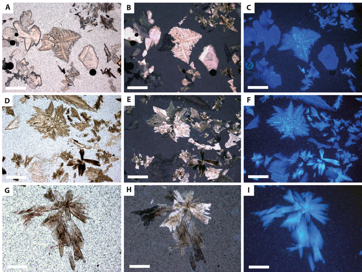
Figure 9. Appearance of cryogenic calcite crystals in thin sections. (a) Dendritic crystal (center) and fragments of rhombohedral crystals nearby as well as smaller aggregates of the white crystal population (e.g., right-hand upper corner of image). Plane-polarized light. (b) Same under partially cross-polarized light. (c) Same under epifluorescence. In (a–c) black rounded spots are air bubbles in the epoxy resin. (d) Mixture of aggregates of rhombohedral crystals, spear-like aggregates (partially visible near upper margin of the image) and few aggregates of the white crystal population (lower right corner). (e) Same under cross-polarized light. (f) Same under epifluorescence. (g) Close-up of a rosette-like aggregate of the white crystal population, which appears brown and rich in minute inclusions in transmitted light. (h) Same under partially cross-polarized light. (i) Same under epifluorescence. Scale bars are 500 \mu\text{m} in (a–f) and 200 \mu\text{m} in (g–i). (a–c) is sample MSK5 and the remaining images are from sample MSK6.
