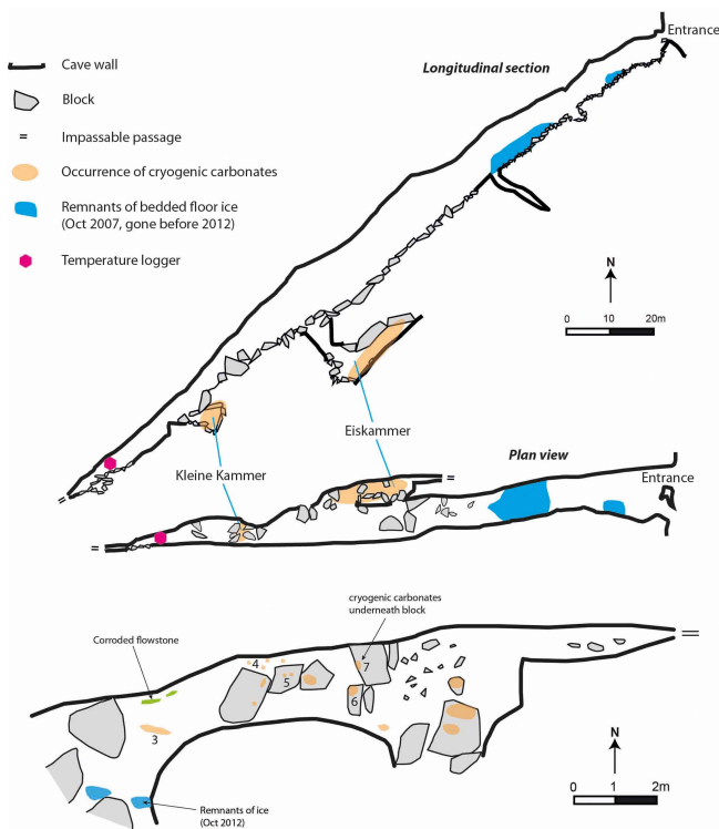
Figure 3. Longitudinal section and plan view of MSK Cave, showing the occurrence of CCC coarse (light brown), and enlargement of the plan view of the Eiskammer (lower panel). Cave survey by C. Spötl and G. Moseley. Numbers refer to samples of CCC coarse sampled in this study, whereby MSK1 and 2 were obtained from the Kleine Kammer and MSK3 to 7 from the Eiskammer.
