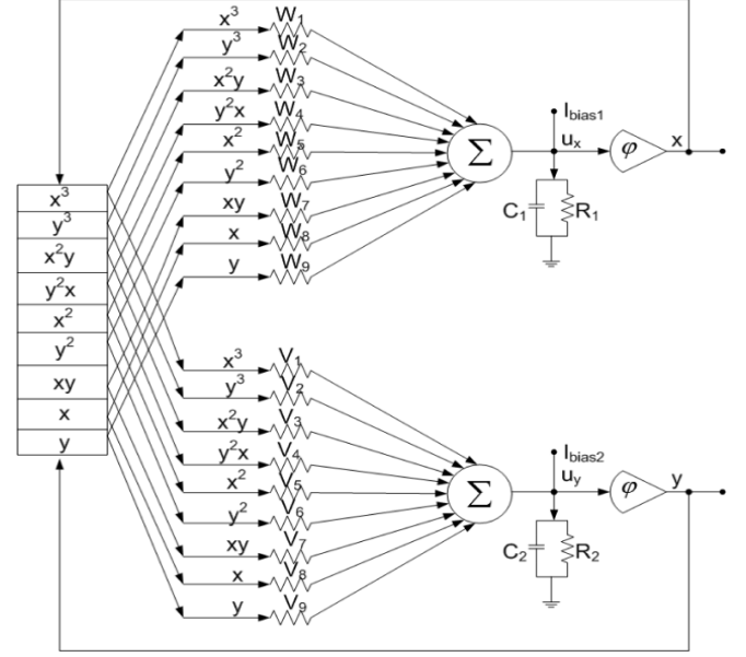
Fig.2. Architecture of the modified Hopfield neural network for Example 1
