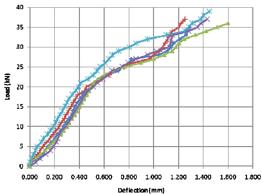
Fig.8. Load-Deflection Curve (three months)
