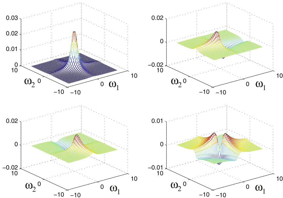
Fig. 5. The real part (top left) and imaginary i -part (top right), j -part (bottom left), and k -part (bottom right) of the output r_2(\cdot) in Example 4.1, i.e. the QFT (70) of (69).
