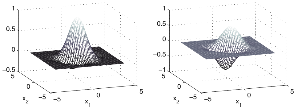
Fig. 1. Representation of the complex Gabor filter for \sigma_1 = \sigma_2 = 1, u_0 = v_0 = 1 in the spatial domain with its real part (left) and imaginary part (right).
