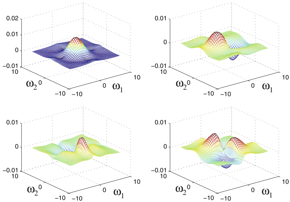
Fig. 6. The real part (top left) and imaginary i -part (top right), j -part (bottom left), and k -part (bottom right) of the output r_1(\omega, \mathbf{b} = 0) in Example 4.2, i.e. the QWFT (71) of (62) with b_1 = b_2 = 0 .
