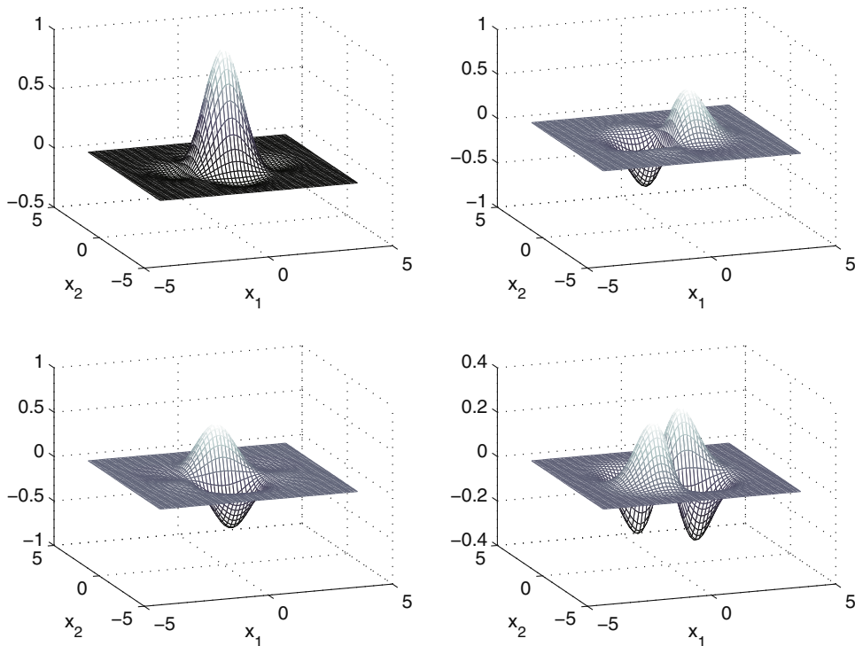
Fig. 2. Bülow's quaternionic Gabor filter (13) ( \sigma_1 = \sigma_2 = 1, u_0 = v_0 = 1 ) in the spatial domain with real part (top left) and imaginary i -part (top right), j -part (bottom left), and k -part (bottom right).
