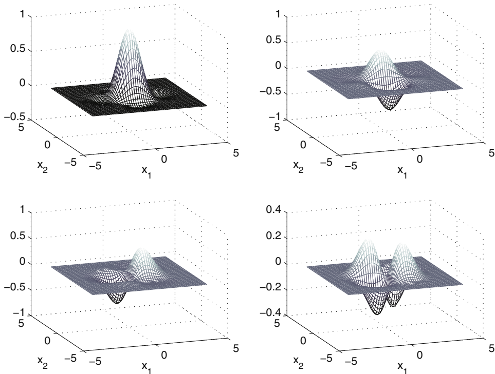
Fig. 3. The real part (top left) and imaginary i -part (top right), j -part (bottom left), and k -part (bottom right) of a quaternionic Gabor filter ( \sigma_1 = \sigma_2 = 1, u_0 = v_0 = 1 ) in the spatial domain.
