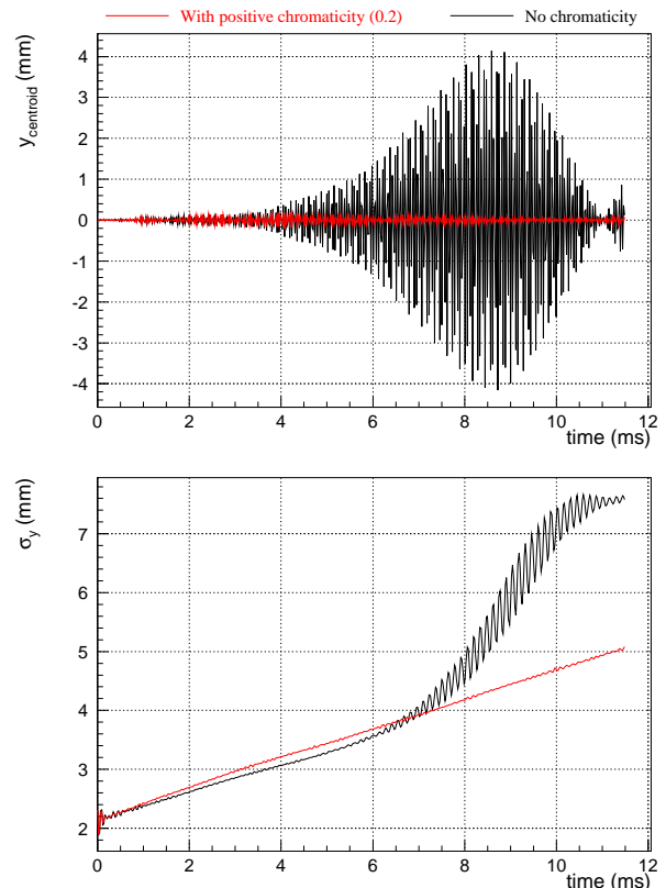
Figure 4: Centroid motion and beam vertical size evolution with and without positive chromaticity (broad-band impedance included).
