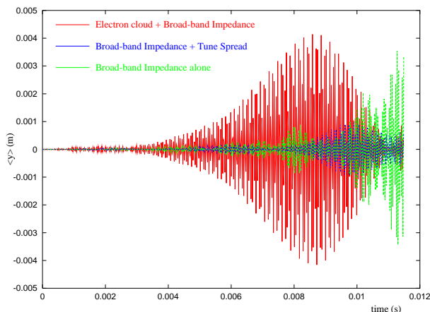
Figure 3: Evolution of the centroid vertical position of an SPS bunch over 500 turns for three different cases.
