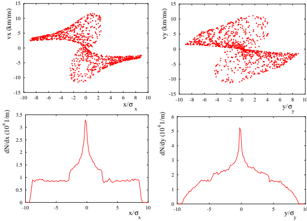
Figure 1: Horizontal and vertical phase space of the electrons after a bunch has gone through (top pictures), and relative distributions (bottom pictures).
