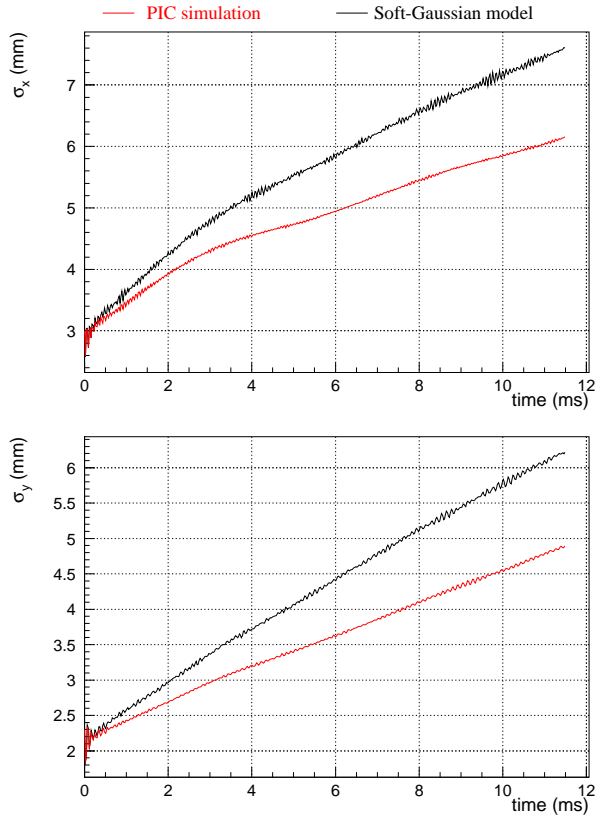
Figure 2: Beam size evolution for an SPS bunch as predicted by PIC and soft-Gaussian simulation ( N_b = 10^{11} )
