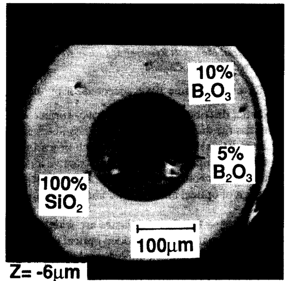
FIG. 4. Acoustic micrograph at z = -6 \mu\text{m} .
