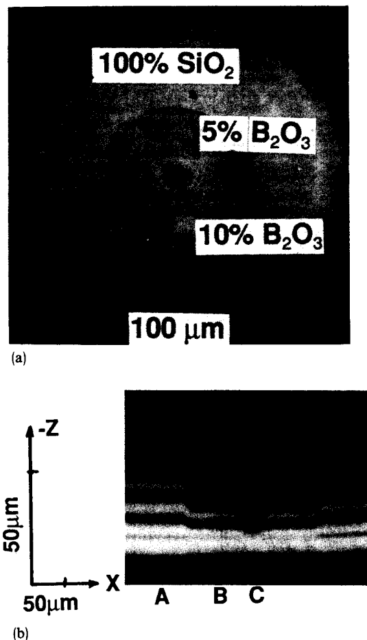
FIG. 1. (a) Transmission optical micrograph of a cladded glass fiber, (b) V(x,z) plane across the center of fiber in (a).
