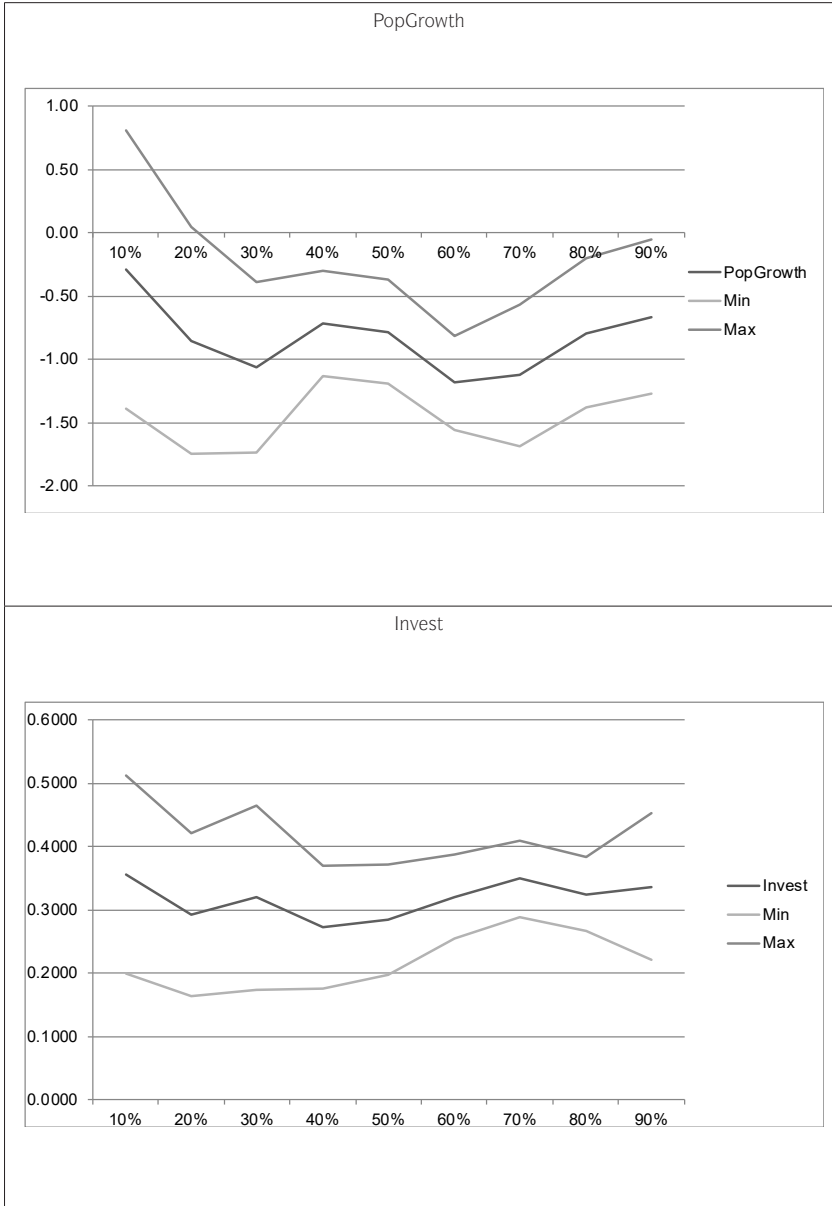
FIGURE 1. QUANTILE RESULTS.
