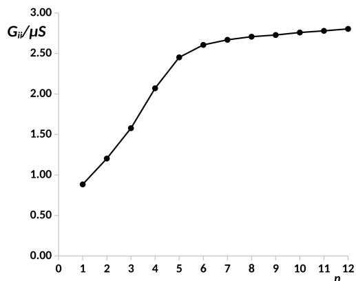
Fig. 2 Electric conductance in the main transport channel, G_{ii} , in \mu S , under a bias voltage of 2V vs number of phenyl units, n , in the pX2 chain as represented in Fig. 1. Data for n=1-8 taken from Ref 34 .
