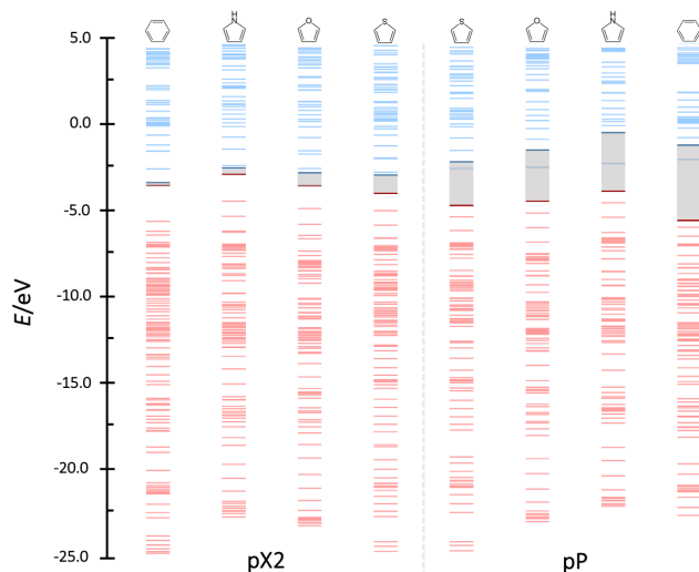
Fig. 10 Orbital bands for the phenyl, pyrrole, furan and thiophene pX2 and pP like chains as represented in Fig. 1 with n=7 . Red and blue colors represent occupied and virtual bands, respectively, whereas the occupied and virtual orbitals involved in the main transmission channel are represented by bold lines.
