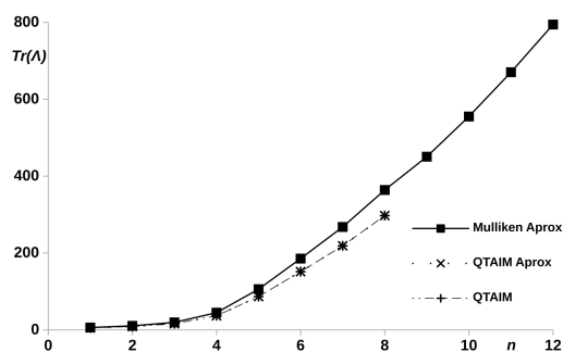
Fig. 6 Trace of the LT calculated for the methylene carbons with the Mulliken and QTAIM atomic partitionings, using eqn (11) and eqn (12) vs number of phenyl units, n , in the pX2 chains
