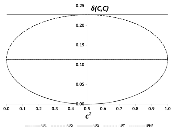
Fig. 12 DIs between the methylene carbon atoms, \delta(C,C) , in the pX2 chain with n=7 vs the relative weight of the H^2 and L^2 configurations, c^2 , for the states represented in Fig. 11 and the Hartree-Fock (HF) result.
