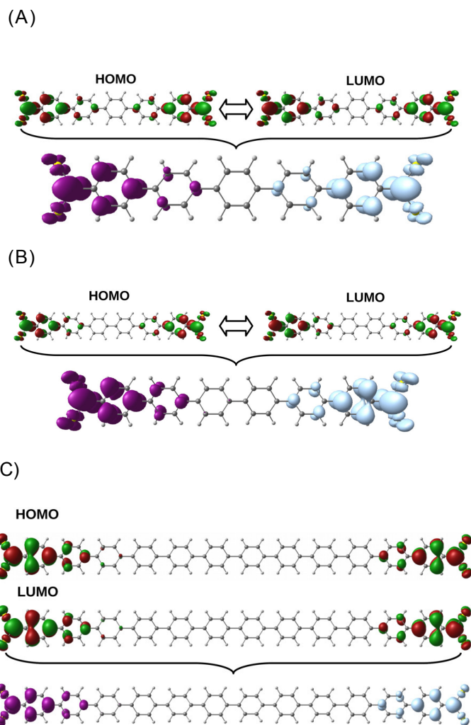
Fig. 3 Distribution of the HOMO-LUMO orbitals and the main transmission channel in the pX2 chain as represented in Fig. 1 with n=5 (A) n=6 (B) and n=12 (C). The isosurface values were 2.5E-2 for the HOMO-LUMO orbitals and 2.5E-3 for the transmission channels. (A) taken from Ref. 16
