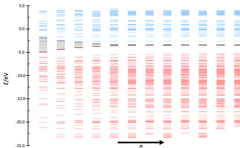
Fig. 8 Orbital bands of the phenyl pX2 structures as represented in Fig. 1 from n=1-12 . Red and blue colors represent occupied and virtual bands, respectively, whereas the occupied and virtual orbitals involved in the main transmission channel are represented by bold lines.
