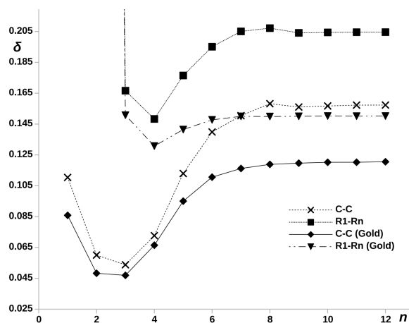
Fig. 5 DI, \delta , between terminal rings, denoted as R_1-R_n , and the methylene carbons denoted as C-C with and without gold electrodes vs number of phenyl units, n , in the pX2 chains. \delta_{R_1-R_2} , being a direct covalent interaction between rings, is out of the bounds of the scale and has been left out of the plot.
