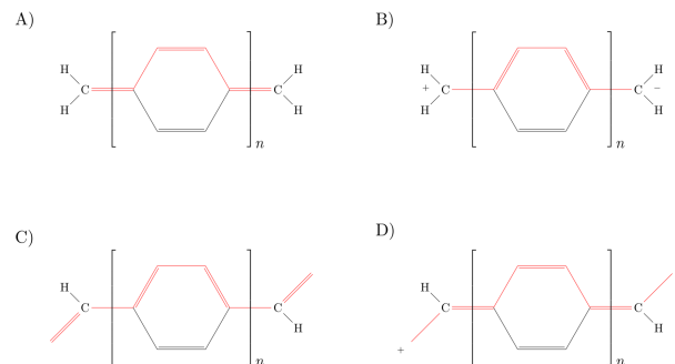
Fig. 7 Resonant forms of pX2 structures: A) trivial , B) topological and pP structures: C) trivial , D) topological . The main polyacetylene structures are depicted in red and the bridging ethylene units in black
