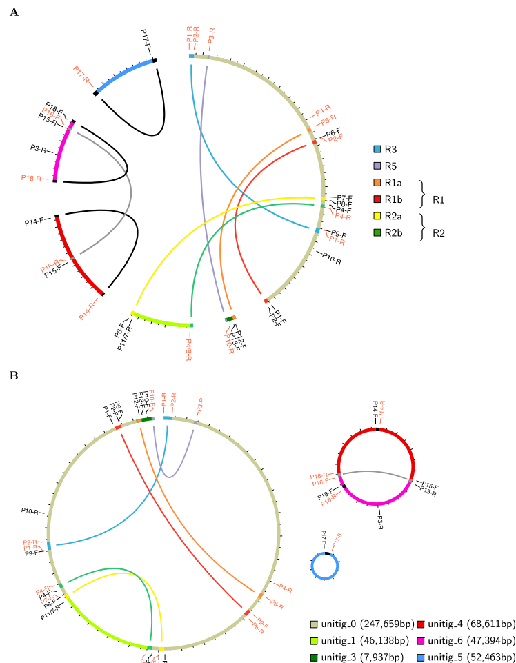
Figure 1. S. tuberosum mitochondrial genome assembly. (A) The 6 unitigs output by HGAP for the Cicero mitogenome. Colored blocks on the unitigs show repeats. Labeled ticks give primers positions, with those in black in forward orientation and those in light red in reverse orientation. (B) The 3 contigs obtained after PCR validation. Colored blocks on the contigs show repeats. The larger contig could not be circularized.
