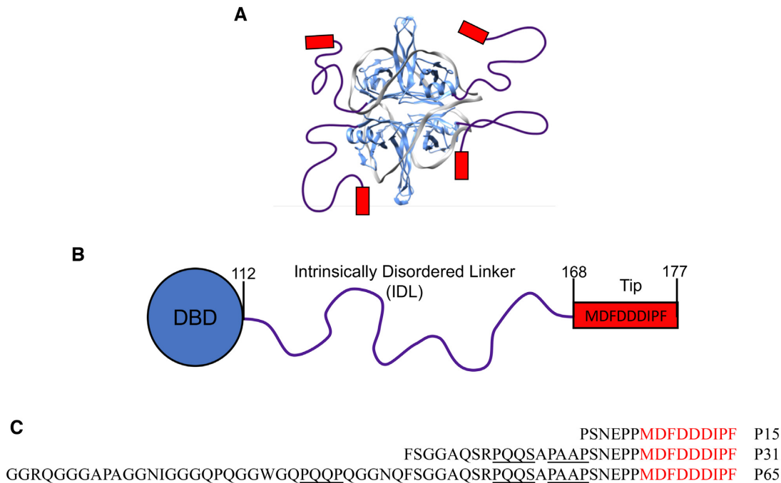
Figure 1. Structure of Escherichia coli SSB. (A) Model for the structure of an SSB tetramer complexed with (dT) 70 in the (SSB) 65 binding mode (1). The IDL (purple lines) and the nine amino acid acidic tips (red boxes), are shown schematically. (B) A cartoon representation of the domain structure of an SSB subunit showing the N-terminal DNA binding domain (DBD) (residues 1–112), the 56 amino acid IDL (residues 113–168) and the acidic tip (residues 169–177). (C) Sequences of the SSB-Ct peptides with the PXXP motifs underlined in black.
