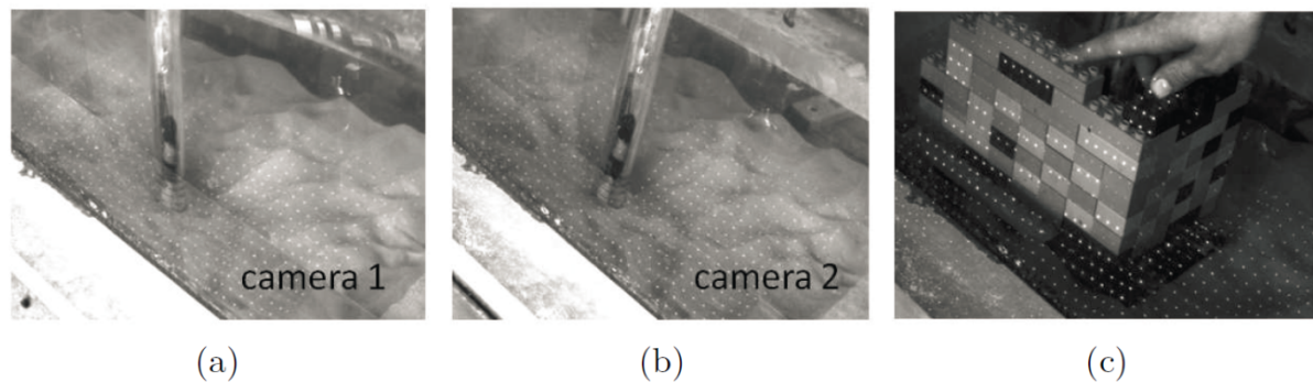
Figure B.2. (a) and (b): stereo pairs related to the experimental settings. The projected laser dots onto the sandy bottom and the the scour around a vertical pile are visible. (c) 3D rig used during calibration.
