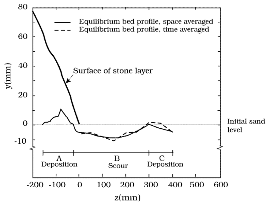
Figure 2.13. Mean bed profile, space- and time averaged in cross-flow direction. Sketch of scour and deposition pattern. Live-bed ( \theta > \theta_{cr} ). Test 9. Vertical scale is grossly exaggerated.
