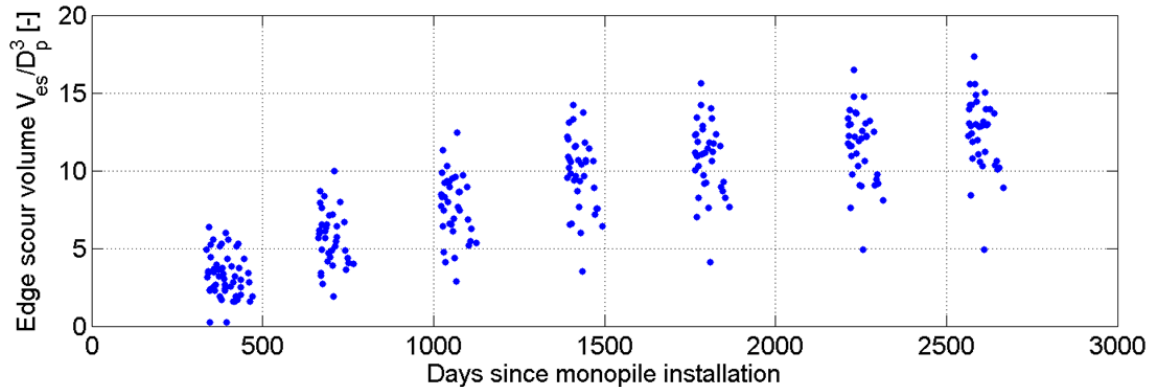
Figure 3.36: Edge scour development in time in NNE-octant (radially averaged over the area between 0^\circ\text{N} and 45^\circ\text{N} and averaged over all monopiles; normalized by the pile diameter)
