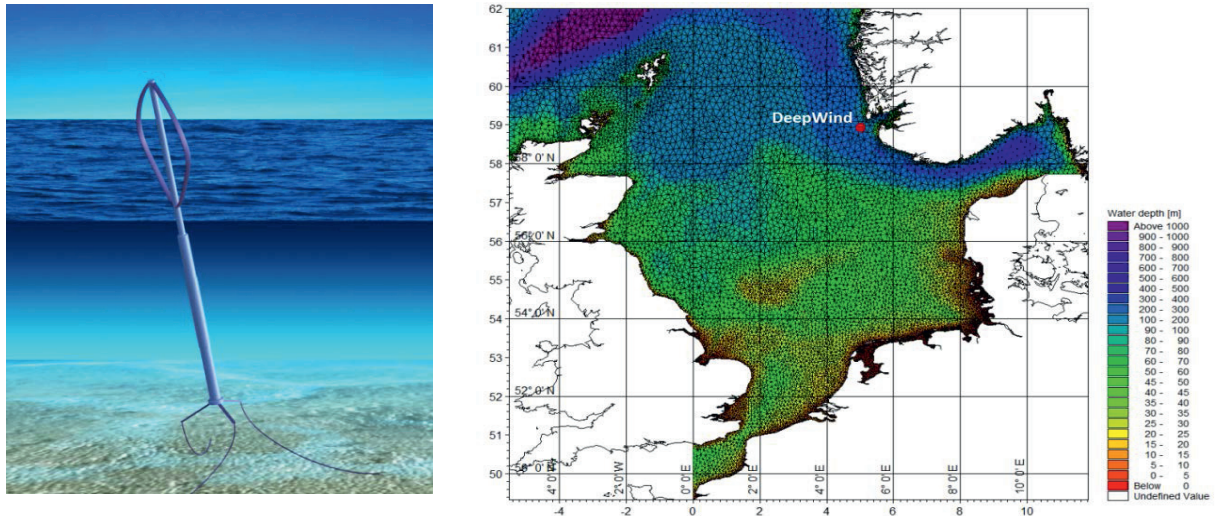
Figure 1 Left: DeepWind, the Vertical-Axis Darrieus concept for deep sea concept. Right: Approximate position of the DeepWind turbine evaluation site[1], Latitude: 59^{\circ} 8'44.88''\text{N} , Longitude: 5^{\circ} 1'25.66''\text{E} (from DHI's Hindcast model)
