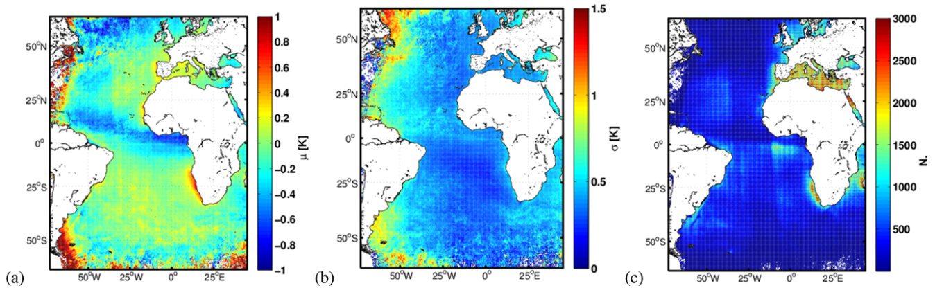
Figure 1. SEVIRI–AATSR (a) mean bias \mu , (b) standard deviation \sigma , (c) number of match-ups N , binned in 25 \text{ km} \times 25 \text{ km} boxes.
