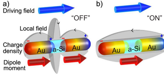
FIG. 1: Illustration of the principle of antenna switching using a photoconductive gap, showing the fundamental mode of an unswitched ("OFF") (a) and a switched ("ON") (b) nanoantenna.
