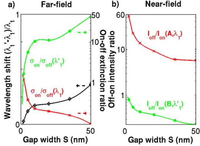
FIG. 5: Figures of merit for switching operation for operation in far-field (a) and near-field (b). (a) Relative resonance shift (\lambda'_1 - \lambda_1)/\lambda_1 (left scale, linear) and on-off extinction ratio \sigma_{on}/\sigma_{off} at wavelengths \lambda_1 and \lambda'_1 (right scale, logarithmic), against antenna gap width S . (b) Near-field intensity off-on ratios I_{off}/I_{on} at \lambda_1 , point A (midgap) and \lambda'_1 , point B (5 nm from tip).
