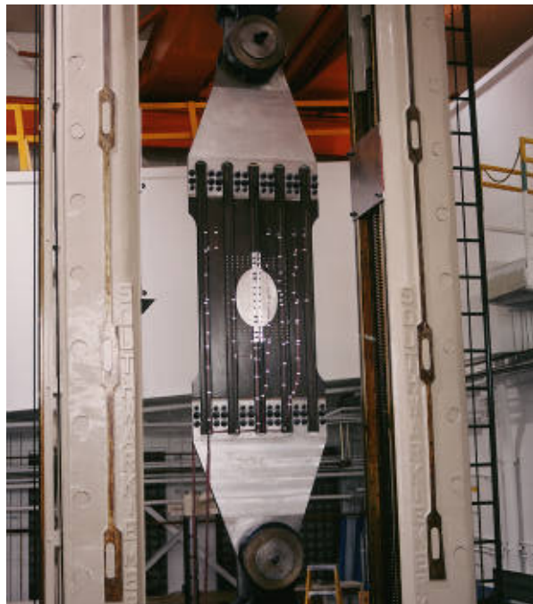
Figure 22b. Stitched/RFI wing panel in Langley 1,200-kip machine for damage repair test.
