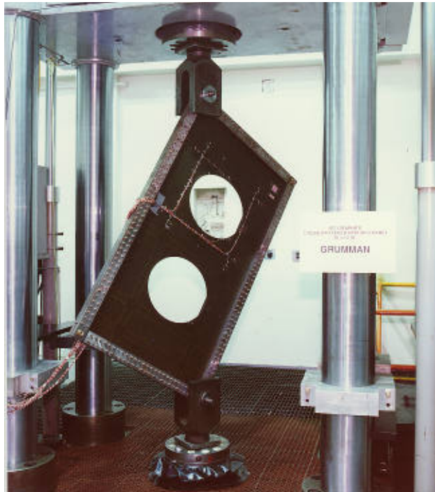
Figure 20. Picture frame shear test of cross-stiffened fuselage window belt component.
