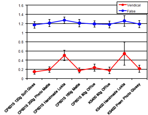
Figure 4. Plots mean SDED values and standard deviation error bars for veridical and false matches for each paper/print combination. The sigma of Gaussian smoothing was 5.0.
