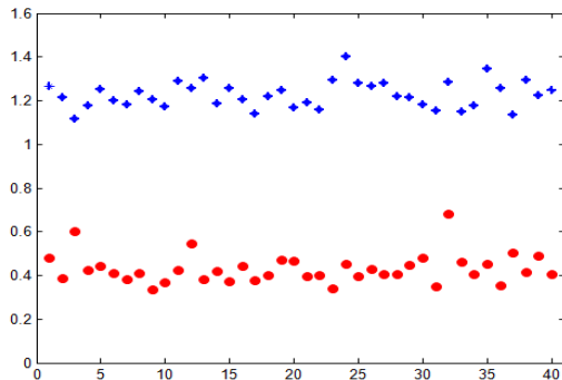
Figure 3. Plots SDED values for 40 veridical matches (red) and 40 random false matches (blue) for CP6015 laser print on 80g office paper. The sigma of Gaussian smoothing was 5.0.
