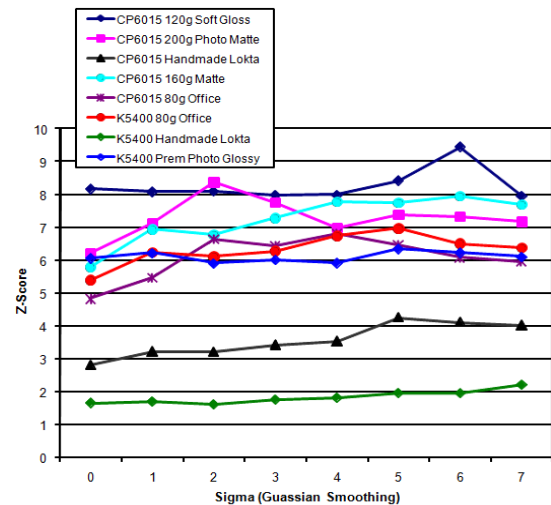
Figure 5. Plots approximate Z-score trend against the Sigma used in low-pass filter for each paper/print combination.
